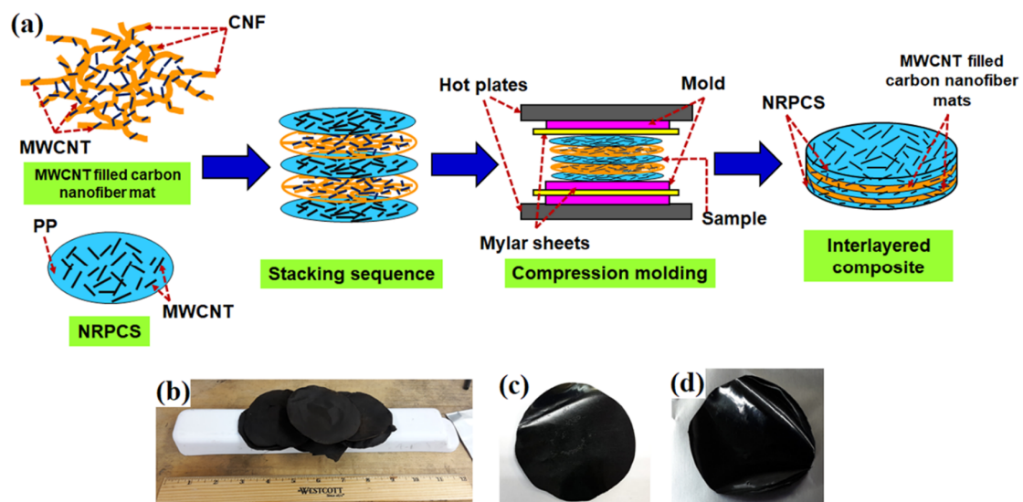
Figure 1. (a) Schematic representation of the fabrication process of interlayered composites; Digital pictures of (b) MWCNT filled carbon nanofiber mats; (c) NRPCS used as starting materials; and, (d) a resultant one-layer interlayered flexible composite.
