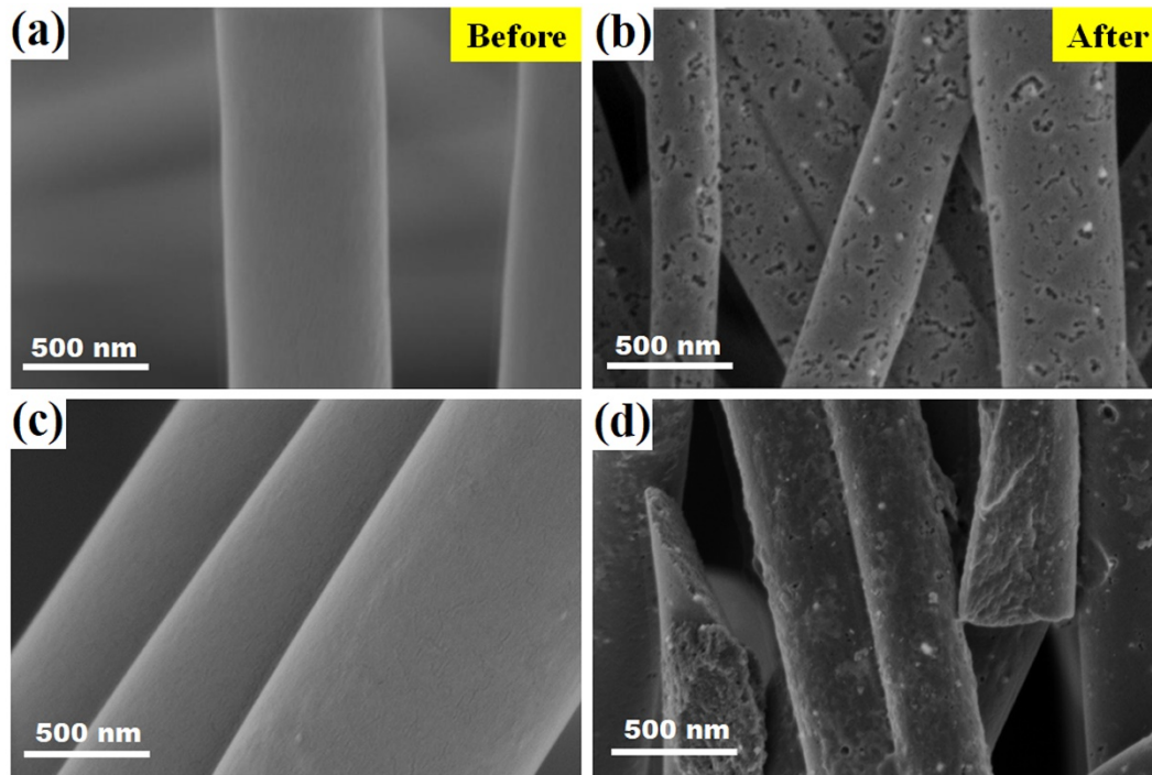
Figure 4. SEM images of MWCNT filled carbon nanofiber mats with different contents of MWCNT before and after carbonization. (a,c) PVA nanofibers mats with 0.05 and 0.1 wt.% MWCNT and (b,d) CNF mats filled with 0.05 and 0.1 wt.% MWCNT, respectively.
