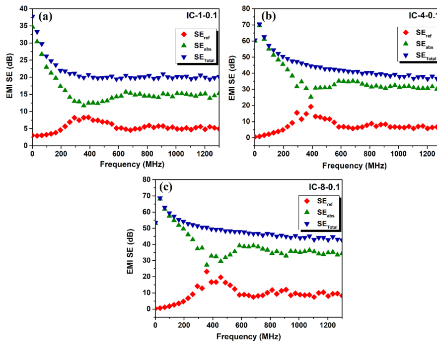
Figure 8. Reflection, SE_{ref} (◆), absorption, SE_{abs} (▲), and total SE, SE_{Total} (▼) for interlayered composites: (a) IC-1-0.1; (b) IC-4-0.1; and, (c) IC-8-0.1.
