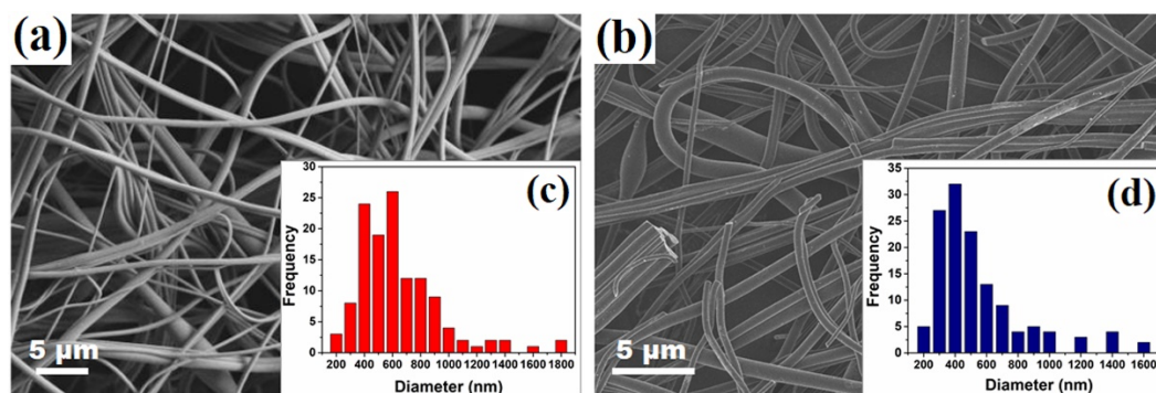
Figure 3. SEM images of (a) nonwoven Poly(vinyl alcohol) (PVA) nanofibers mat and (b) nonwoven carbon nanofibers (CNF) mat without MWCNT. Histograms representing fiber diameter distributions are shown as insets for both systems (c) and (d).
