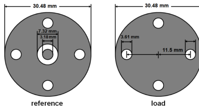
Figure 2. Fixture configuration for testing of electromagnetic interference (EMI) shielding effectiveness [29].
