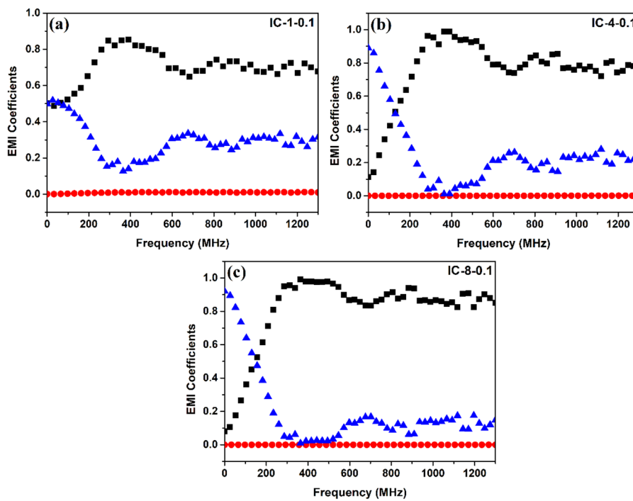
Figure 7. EMI power coefficients of reflectance (■), transmittance (●), and absorbance (▲) of the interlayered composites: (a) IC-1-0.1; (b) IC-4-0.1; and, (c) IC-8-0.1.
