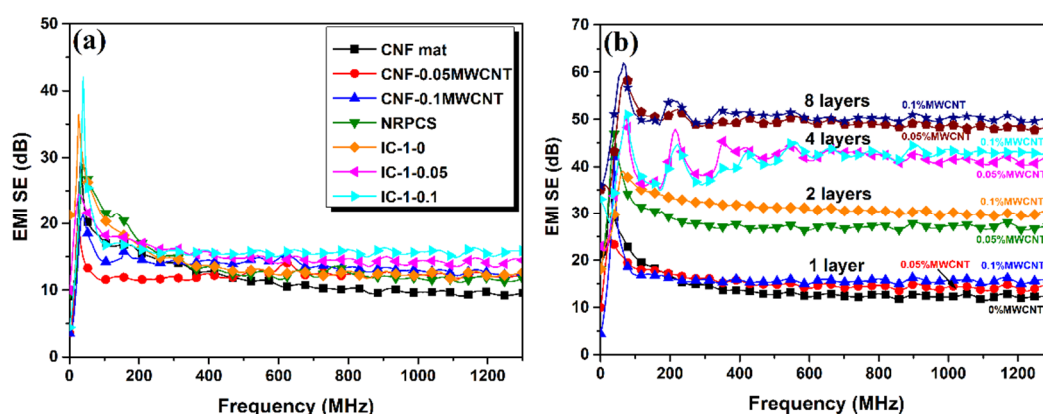
Figure 6. (a) Total experimental EMI shielding effectiveness (EMI SE) of nonwoven CNF mat, NRPCS, MWCNT filled carbon nanofiber mats with different MWCNT contents, and one-layered flexible composites; and (b) EMI SE of interlayered composites formed by different number of layers of MWCNT filled carbon nanofiber mats with variable MWCNT concentration.
