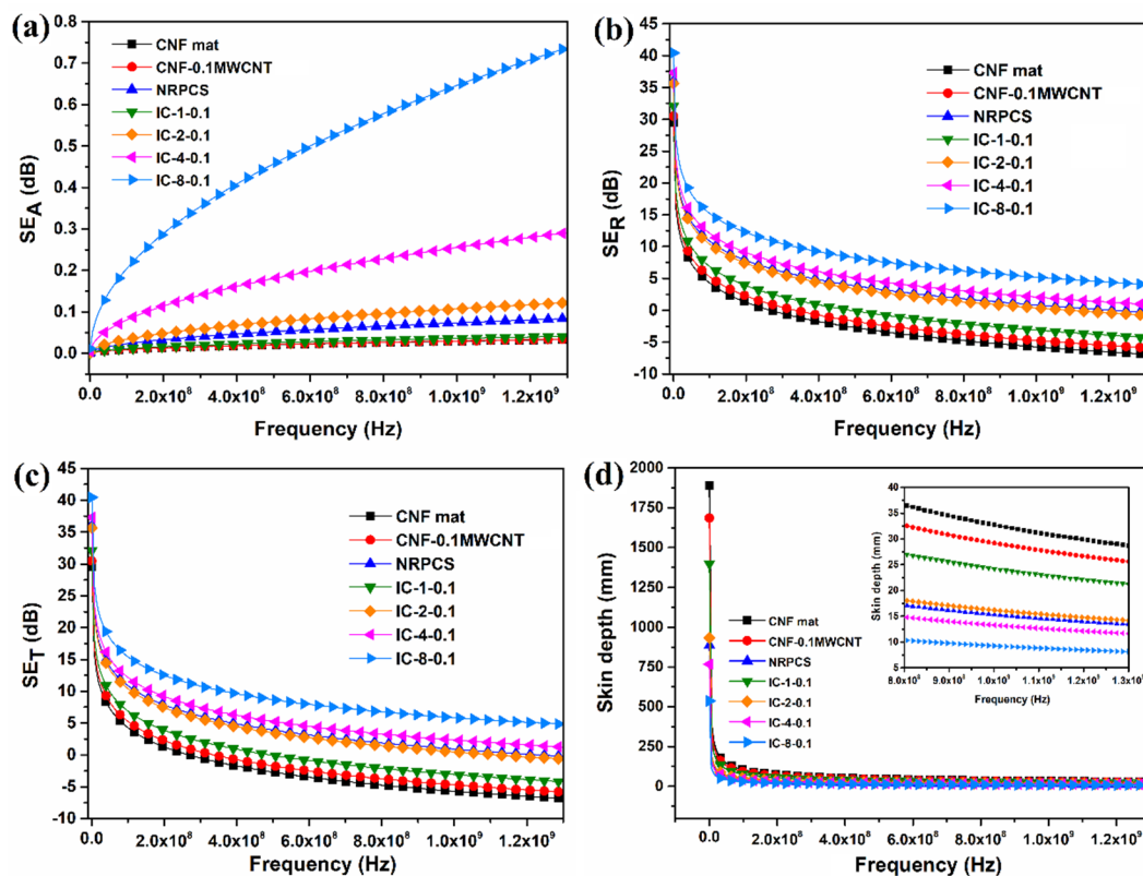
Figure 9. Calculated EMI SE versus frequency. (a) SE_A ; (b) SE_R ; (c) SE_T of CNF mat, 0.1 wt.% MWCNT filled carbon nanofiber mat, NRPCS and interlayered composites formed by different number of layers of 0.1 wt.% MWCNT filled carbon nanofiber mats; and, (d) Skin depth dependence with respect to frequency. The inset in (d) shows a zooming view of skin depth at higher frequencies (0.8–1.3 GHz).
