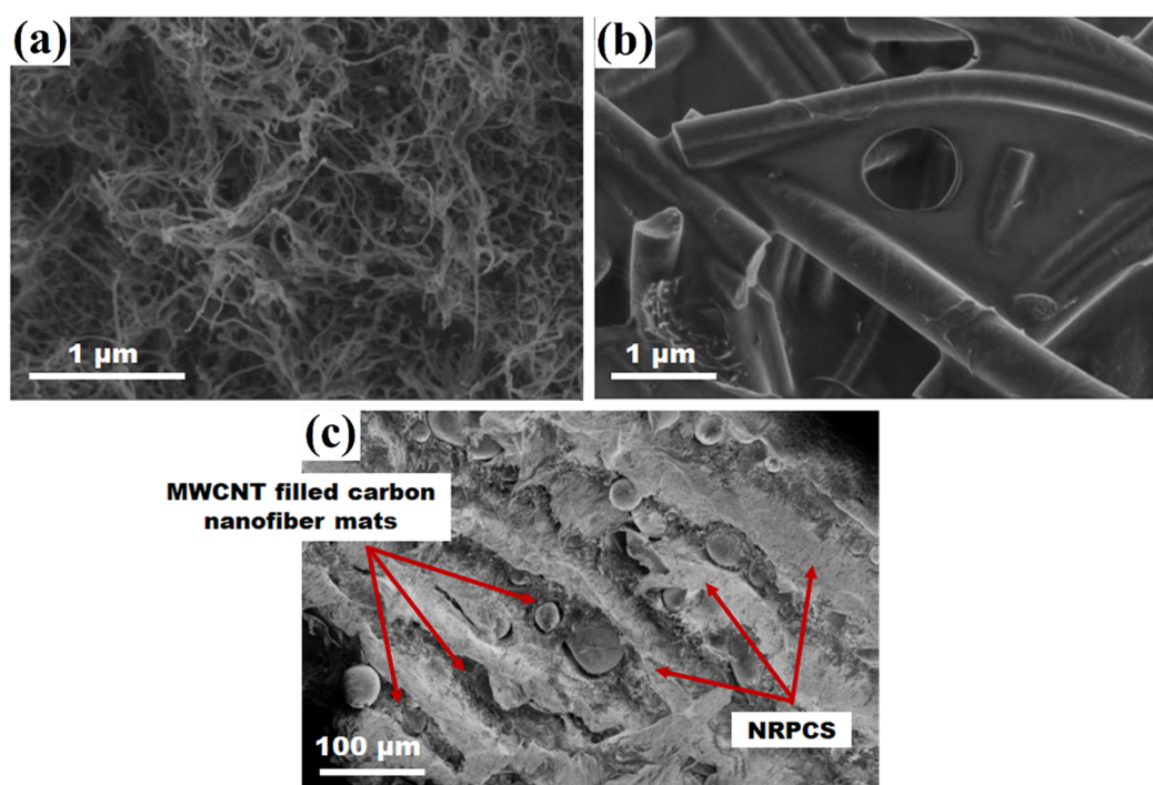
Figure 5. SEM images of (a) a cross-sectional of the NRPCS; (b) MWCNT filled carbon nanofiber mat embedded within the NRPCS; and, (c) the cross-sectional area of an eight-layered flexible composite.
