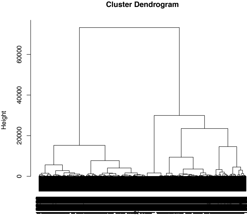
Figure A2: Cluster Dendrogram
