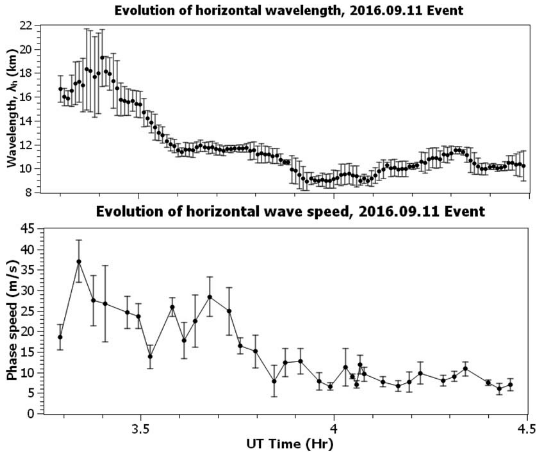
Figure 3. The time variations of the horizontal wavelength (top) and horizontal phase speed (bottom) of the “blocked” wave during the wave “blocking” event. The number of data point of the horizontal phase speed is less than those of the horizontal wavelength, because more frames of AMTM measurements are needed for its calculation.
