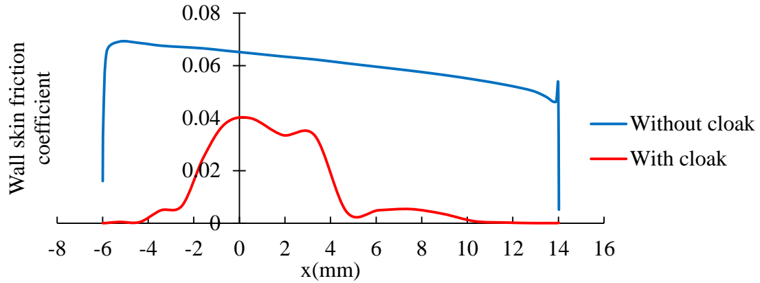
(c) Re=100
