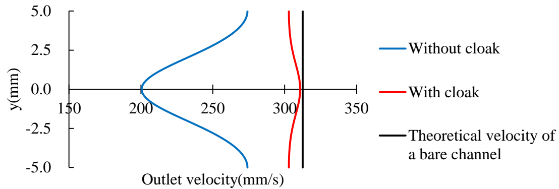
(a) Re=1.5
