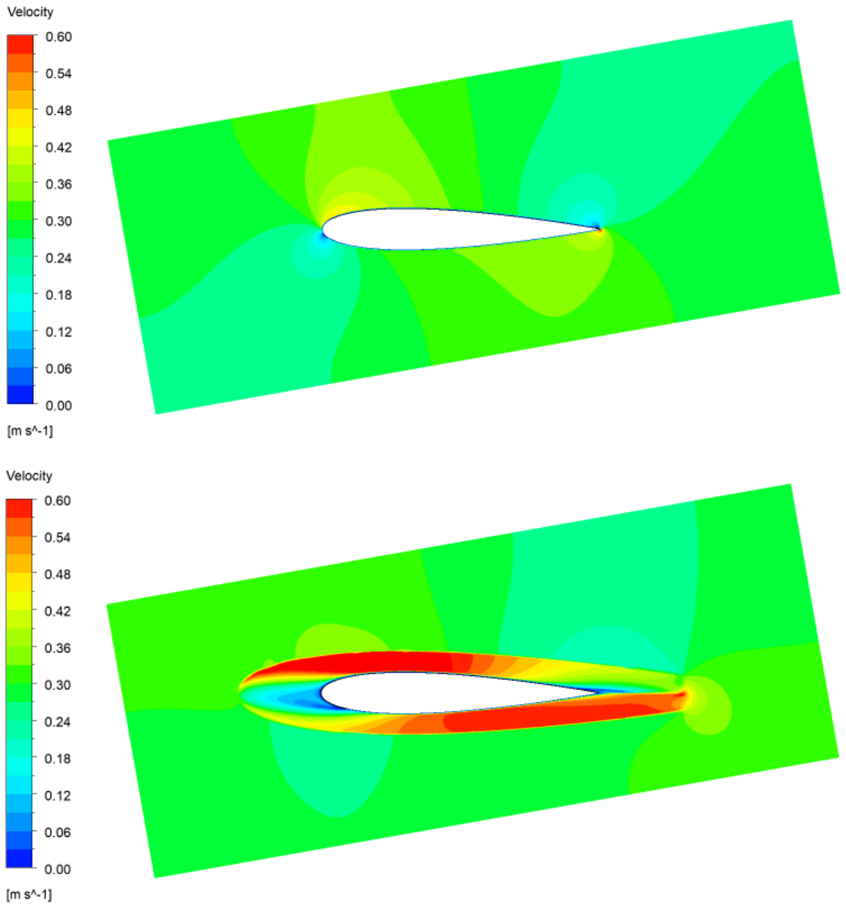
(a) The case without cloak (up) and the case with cloak (down) at Re=1
