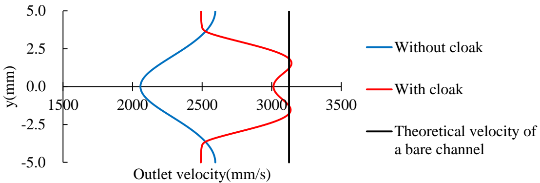
(c) Re=150
