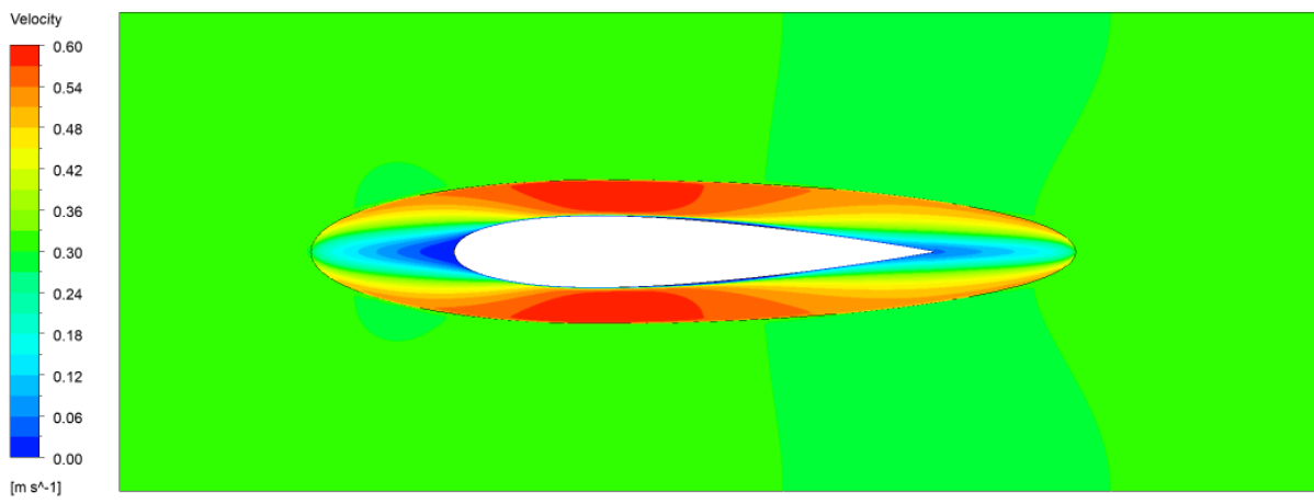
(a) The case without cloak (up) and the case with cloak (down) at Re=1
