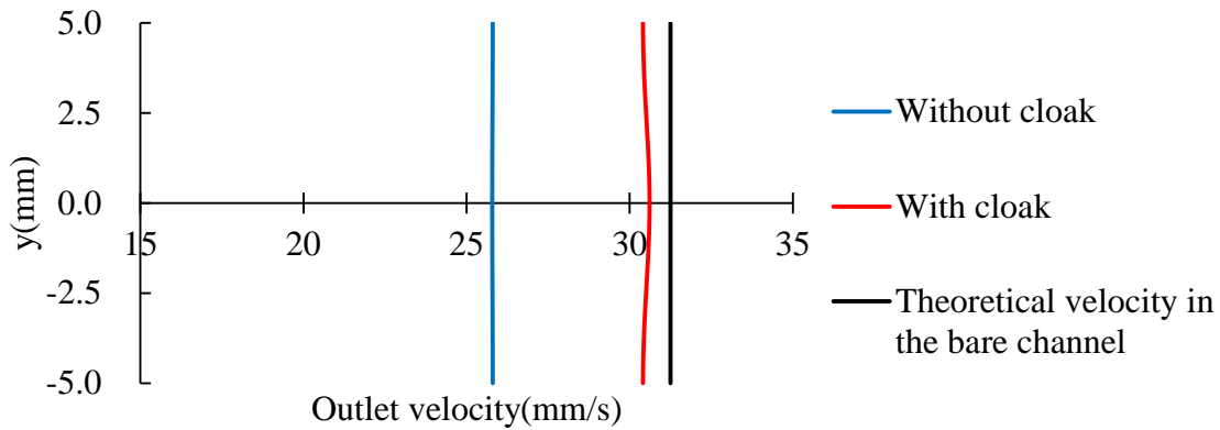
(a) Re=1.5
