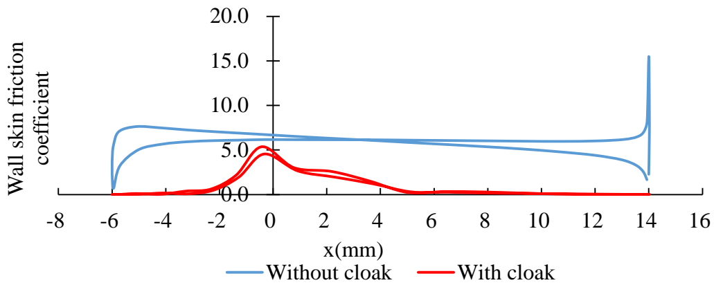
(a) Re=1
