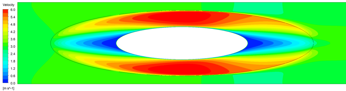
(c) The case without cloak (up) and the case with cloak (down) at Re=150
