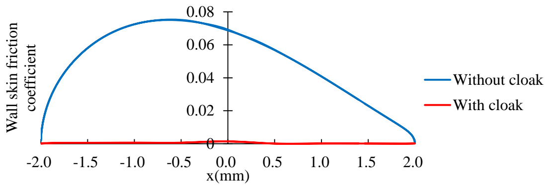
(c) Re=150
