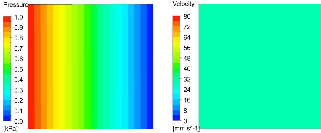
(a) Pressure contours
