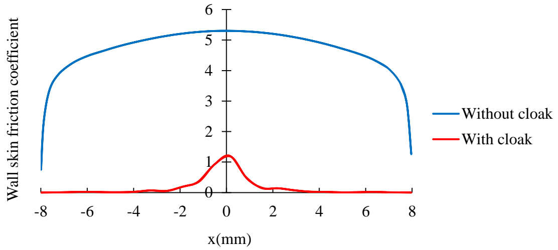
(a) Re=1.5
