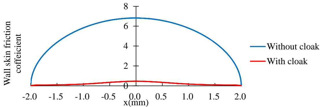
(a) Re=1.5
