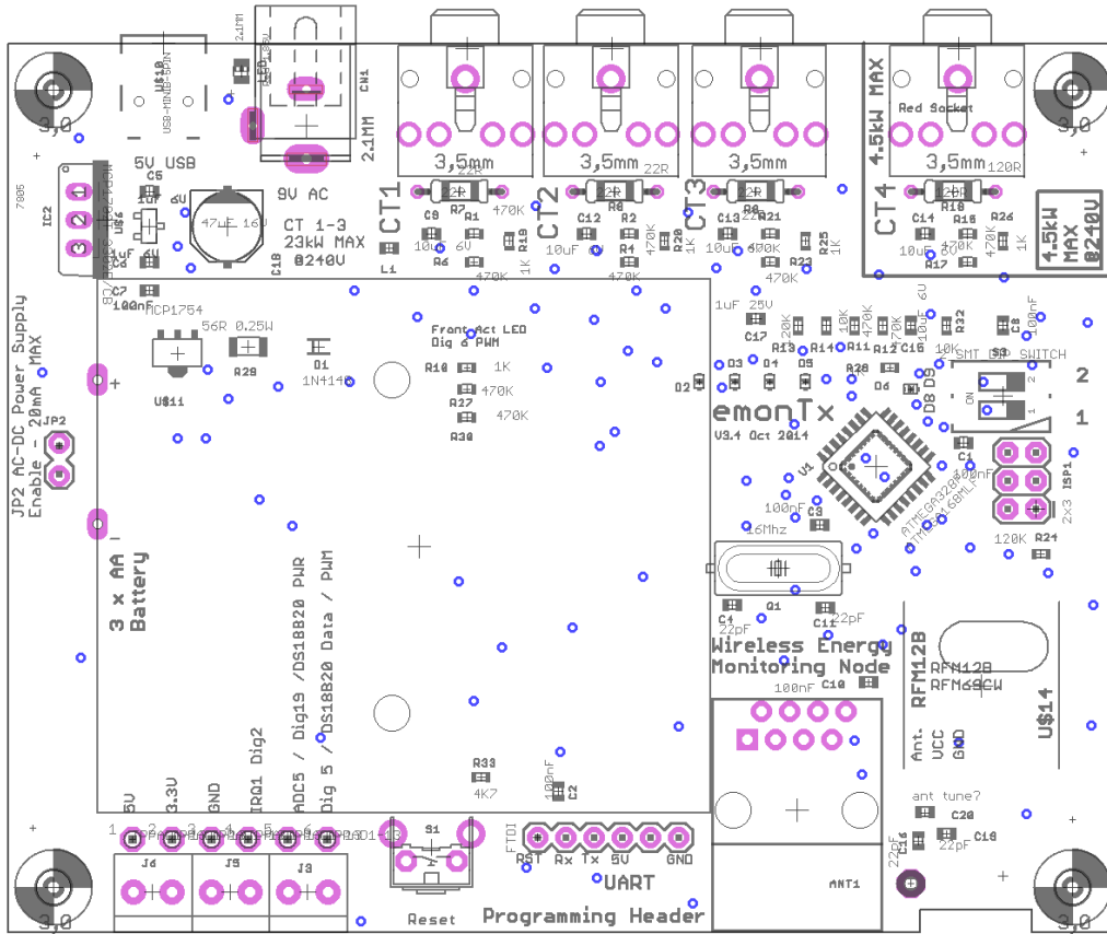
Figure 5: emonTx Board Layout
