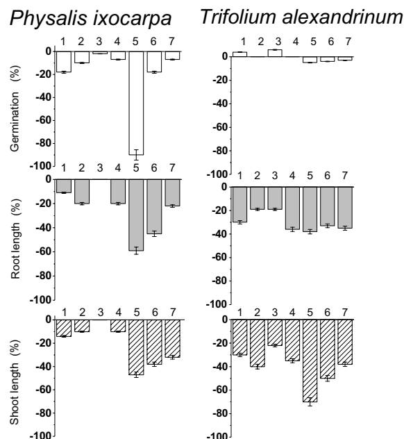
Fig. 3. Effect of lactones 1–7 at 200\ \mu\text{M} on germination, root and shoot length of dicotyledonous species.
