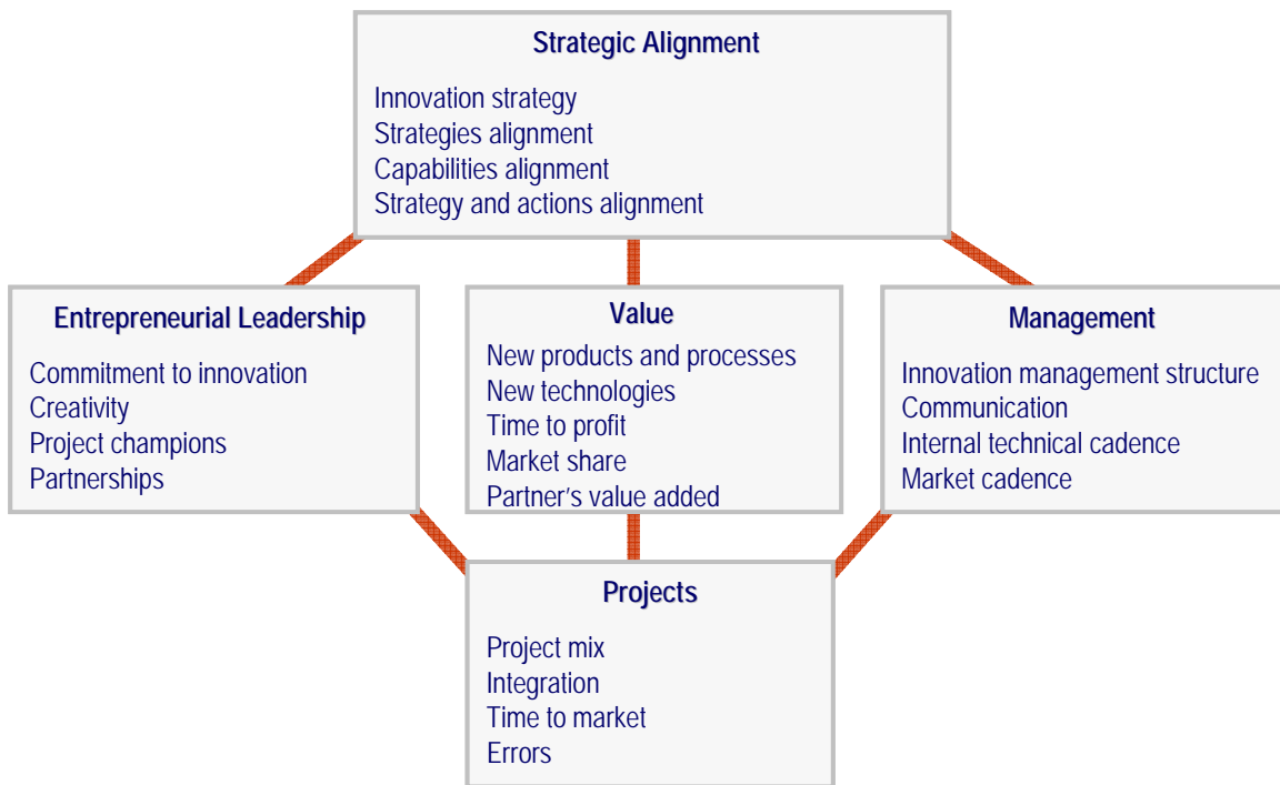
Figure 2. Emerging non-conventional indicators
