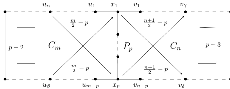
Figure 3. Even and odd cycles merged along a common subgraph
