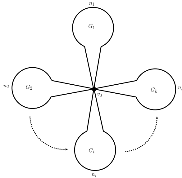
Figure 6. Vertex amalgamation of G_i 's
