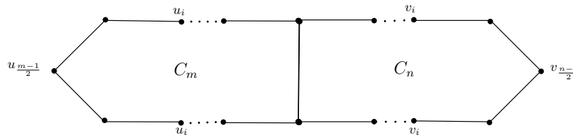
Figure 4. Two odd cycles C_m and C_n identifying a pair of edges
