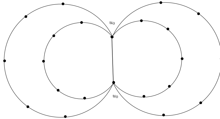
Figure 5. Four 7-cycles sharing a common edge
