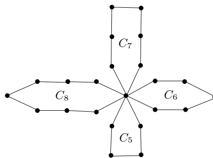
Figure 9. One point union of different cycles
