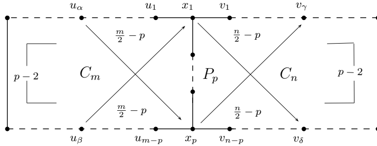
Figure 2. Two even cycles merged along a common subgraph
