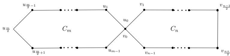
Figure 11. An even cycle C_m and an odd cycle C_n merged at a vertex
