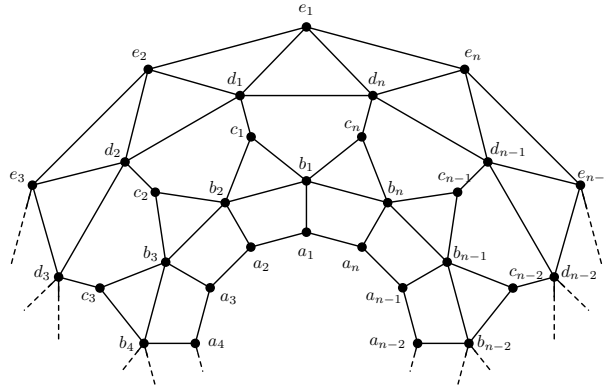
Figure 2. The graph of convex polytope \mathbb{C}_n
