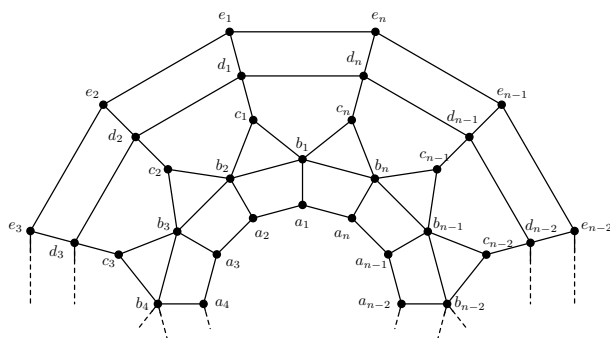
Figure 1. The graph of convex polytope B_n
