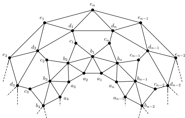
Figure 3. The graph of convex polytope E_n
