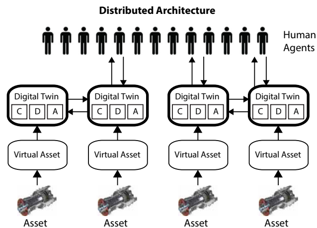
Fig. 4 Block diagram of the Distributed architecture. Black arrows indicate communications between its elements. Human agents and assets are not considered to be part of the software architecture, as they are elements in the physical world. The thicker blocks, pertaining to the Digital Twins, indicate the element of the architecture performing prognostics for the assets in the industrial fleet. C, D, A are used to indicate the Communications manager, the Data Repository and the Analytics engine of the Digital twin
