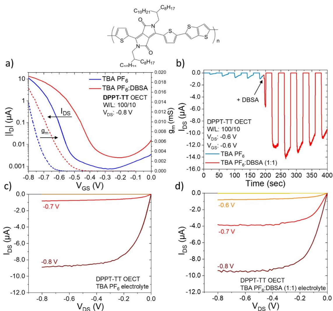
Figure 5. DPPT-TT OECT Operation: (a) transfer characteristics of OECT with TBA PF 6 (blue) and with TBA PF 6 :DBSA (1:1) mixed electrolyte (red) both in ACN; (b) transient gate voltage pulse of OECT with TBA PF 6 (blue) and with DBSA (red) added to the electrolyte mixture; (c) output characteristics with TBA PF 6 electrolyte; (d) output characteristics with TBA PF 6 :DBSA (1:1) mixed electrolyte.
