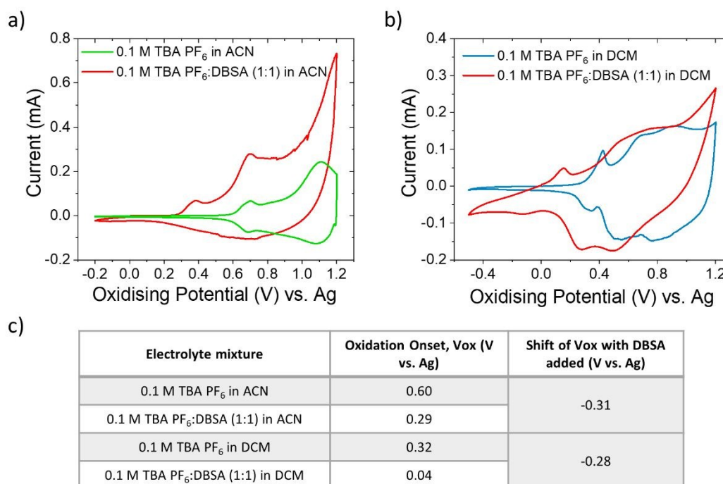
Figure 2. Cyclic voltammograms of P3HT thin films in different electrolytes. (a) TBA PF 6 (green) and TBA PF 6 :DBSA (1:1) mixture (red) in acetonitrile (ACN). (b) TBA PF 6 (blue) and TBA PF 6 :DBSA (1:1) mixture (red) in dichloromethane (DCM). (c) Table summarising the oxidation onsets in each electrolyte mixture.
