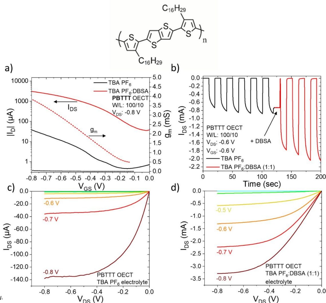
Figure 6. PBTTT OECT Operation: (a) transfer characteristics of OECT with TBA PF 6 (black) and with TBA PF 6 :DBSA (1:1) mixed electrolyte (red) both in ACN; (b) transient gate voltage pulse of OECT with TBA PF 6 (black) and with DBSA (red) added to the electrolyte mixture; (c) output characteristics with TBA PF 6 electrolyte; (d) output characteristics with TBA PF 6 :DBSA electrolyte.
