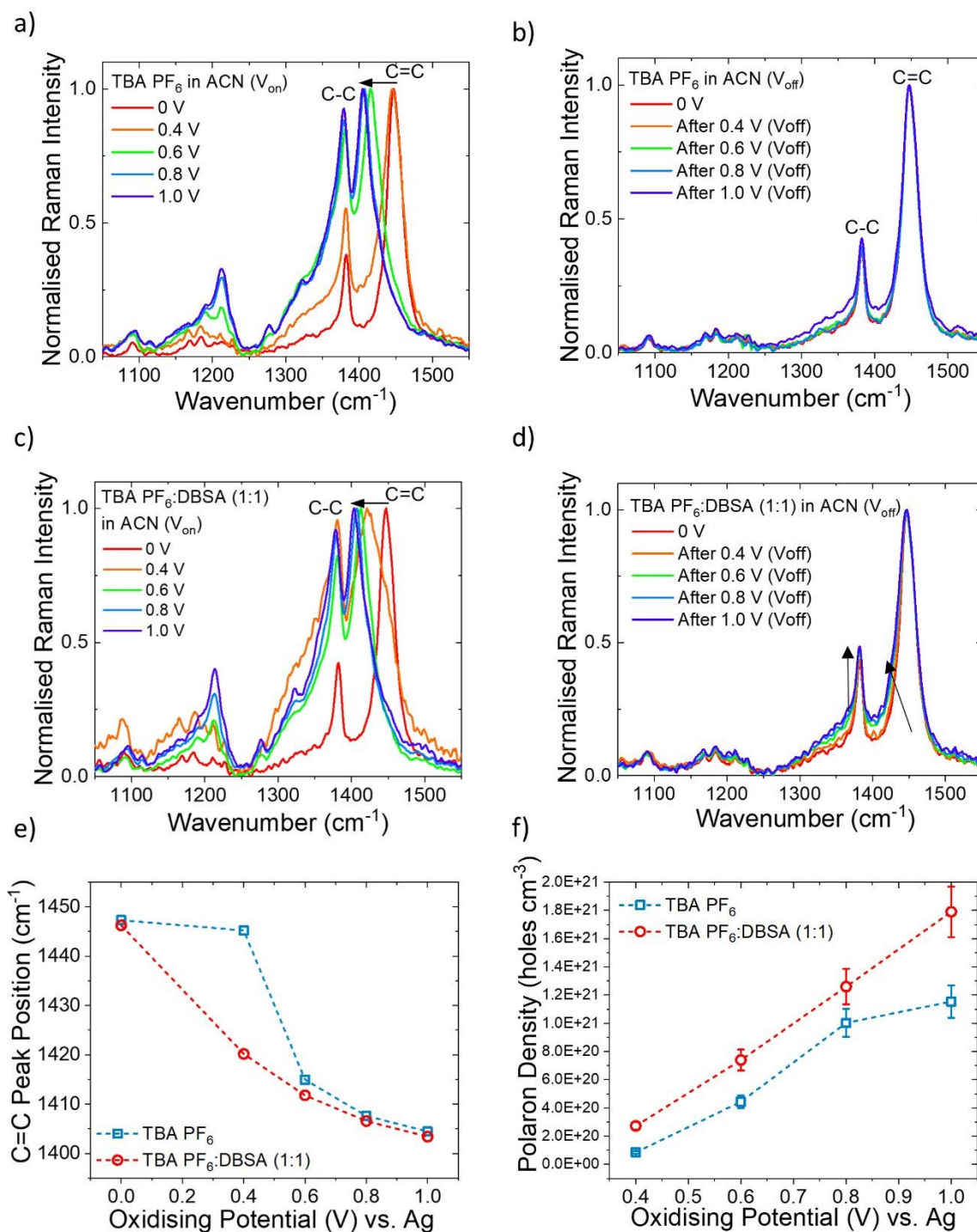
Figure 3. Characterising doping mechanism of TBA PF 6 and TBA PF 6 /DBSA electrolytes: reversible electrochemical doping of TBA PF 6 /DBSA electrolyte mixtures. (a) – (d) in situ ERS measurements with different electrolyte mixtures: 0.1 M TBA PF 6 in acetonitrile, V on and V off (a & b); 0.1 M TBA PF 6 :DBSA (1:1) in acetonitrile, V on and V off (c & d). (e) Peak position of the peak assigned to the C=C vibrational mode as a function of oxidising potential (V). (f) Polaron density generated in the P3HT thin film as a function of oxidising potential (V) with TBA PF 6 (blue) and with DBSA (red) added to the electrolyte mixture.
