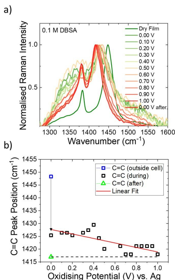
Figure 4. Irreversible chemical doping of DBSA in ACN electrolyte. (a) ERRS spectra of P3HT doped using DBSA in ACN electrolyte. (b) Peak position of the C=C vibrational mode as a function of oxidising potential (V).
