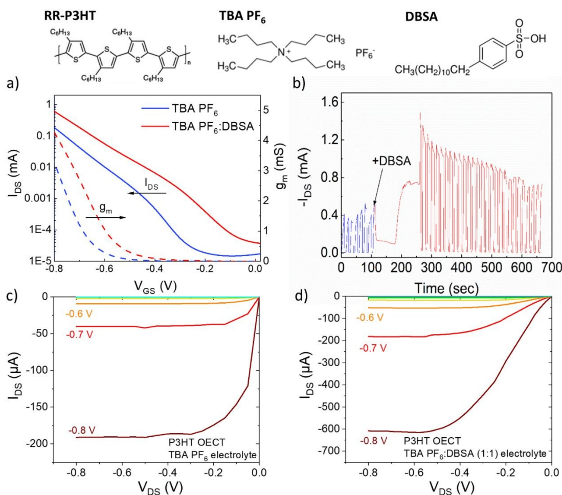
Figure 1. P3HT OECT operation: a) transfer characteristics of OECT with TBA PF 6 (blue) and with TBA PF 6 :DBSA (1:1) mixed electrolyte (red) both in ACN (drain voltage, V_{DS} = -0.8 V); and b) transient gate voltage pulse ( V_{GS} = -0.6 V, V_{DS} = -0.6 V) of OECT with TBA PF 6 (blue) and with DBSA (red) added to the electrolyte mixture; c) output characteristics with TBA PF 6 electrolyte; d) output characteristics with TBA PF 6 :DBSA electrolyte.
