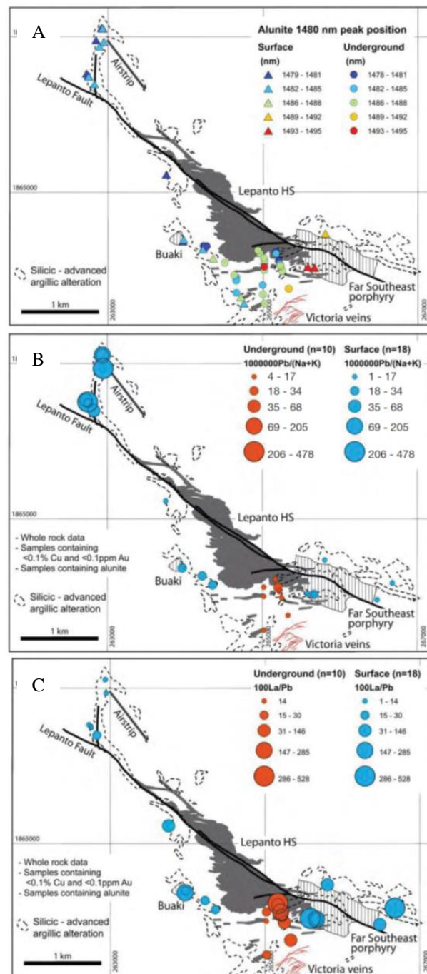
Figure 9: Mankayan lithocap, Philippines. The location of the Lepanto enargite deposit and Far Southeast porphyry copper-gold deposit is shown in grey fill and vertical striped fill, respectively, with surface outcrops of the lithocap marked by dashed lines. (A) Alunite SWIR results. (B) 1000000 * \text{Pb}/(\text{Na}+\text{K}) ratios for whole rock samples. (C) 100 * \text{La}/\text{Pb} ratios for whole rock samples. All whole rock data screened—only alunite-bearing samples with less than 0.1% Cu and 0.1 g/t Au plotted. Diagram modified from Chang et al. (2011).
