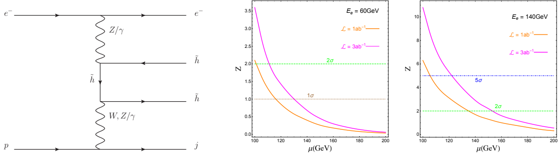
Figure 2: Feynman diagram for Higgsino pair production at an e^- p collider (left). Expected LHeC (center) and FCC-eh (right) reach on Higgsino mass. Taken from ref. [4] and ongoing work.
