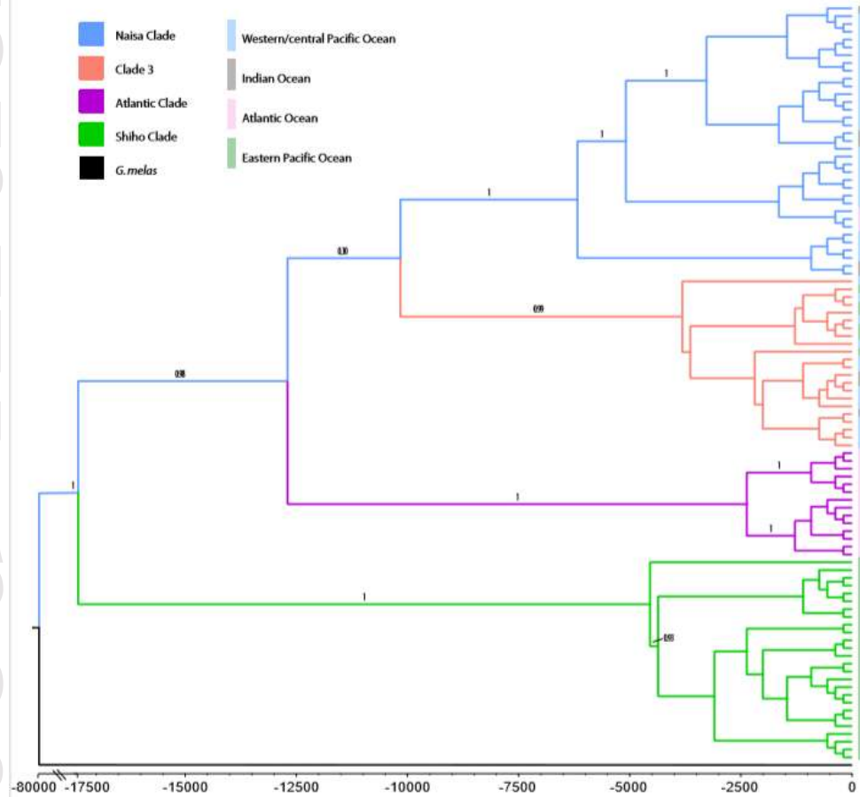
Figure 2. BEAST phylogenetic tree of mitogenome data, rooted with G. melas , showing four distinct clades. The x-axis is Kya. The posterior probability of each branch is shown above the branch, on a scale from 0 to 1. Each branch represents a mitogenome haplotype, which may be shared by multiple individuals. Mitogenome haplotype labels can be seen in Supplemental Figure S2, and mitogenome haplotype frequencies can be found in Supplemental Table S4. The vertical bar on the far right shows the ocean basin where each haplotype was found.
