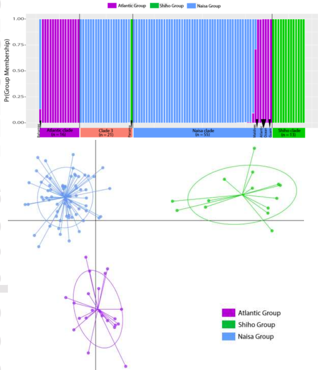
Figure 5. A) Assignment plot based on STRUCTURE analyses, with k = 3 . Mitogenome clade stratification is on the x axis, and probability of assignment is on the y axis. B) Supervised Discriminant Analysis of Principal Components, colored according to the nuclear groups defined in the STRUCTURE analysis in Figure 5A.
