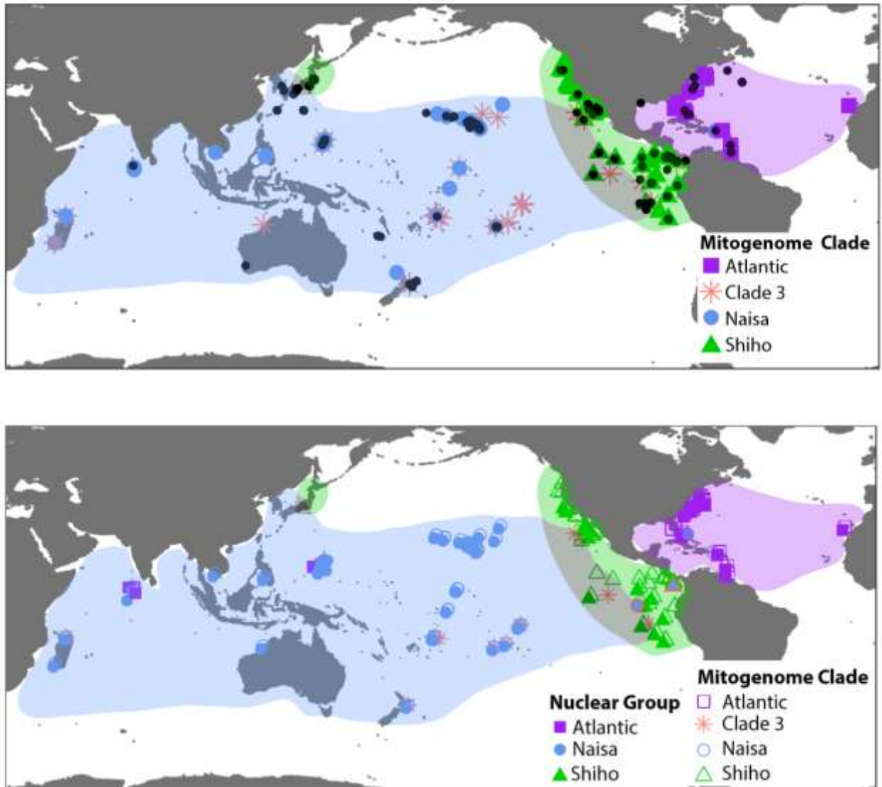
Figure 4. Distributions of A) four mitogenomic clades (black points represent samples for which we have control region samples but no mitogenome or SNP data), and B) three nuclear groups (open shapes represent samples for which we have mitogenome but no nuclear data). Two samples in panel B, outlined in red, are the only eastern Pacific Clade 3 samples with nuclear DNA; one grouped with Naisa, and the other grouped with Shiho. Colored areas in each panel encompass regions of general geographic concordance between the mitogenome and nuclear datasets, which were used to stratify samples into three regions for the estimation of divergence and differentiation among the three hypothesized types. Grey areas show regions of possible sympatry, or regions of recent or historic introgression between types.
