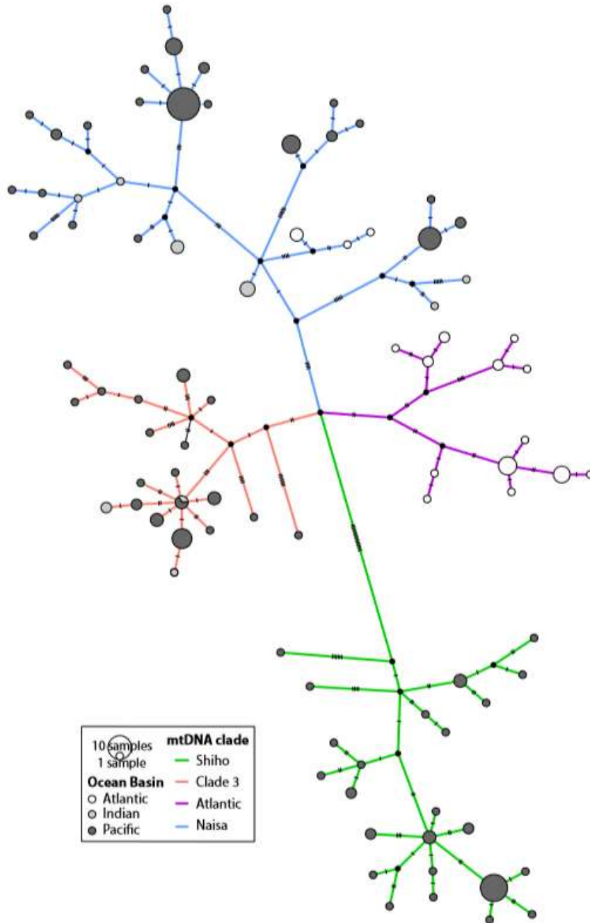
Figure 3. Median joining network (MJN) displaying the relationships among whole mitogenome haplotypes by ocean basin and mitogenomic clades. Circles are proportional in size to the number of samples with each haplotype. Cross hatches on lines indicate the number of differences between haplotypes. Missing haplotypes are indicated by a black node.
