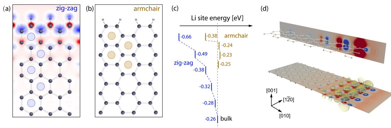
Figure 1. Geometrical structures of graphite edges for zigzag-edged graphite (a) and armchair-edged graphite (b). Periodic boundary conditions were applied in all three directions. (c) is the profile of Li adsorption energies as a function of distance from the edge towards the bulk of graphite. (d) illustrates the spin densities in zigzag-edged graphite. The iso-surface value is 0.0002 e/Å 3 .
