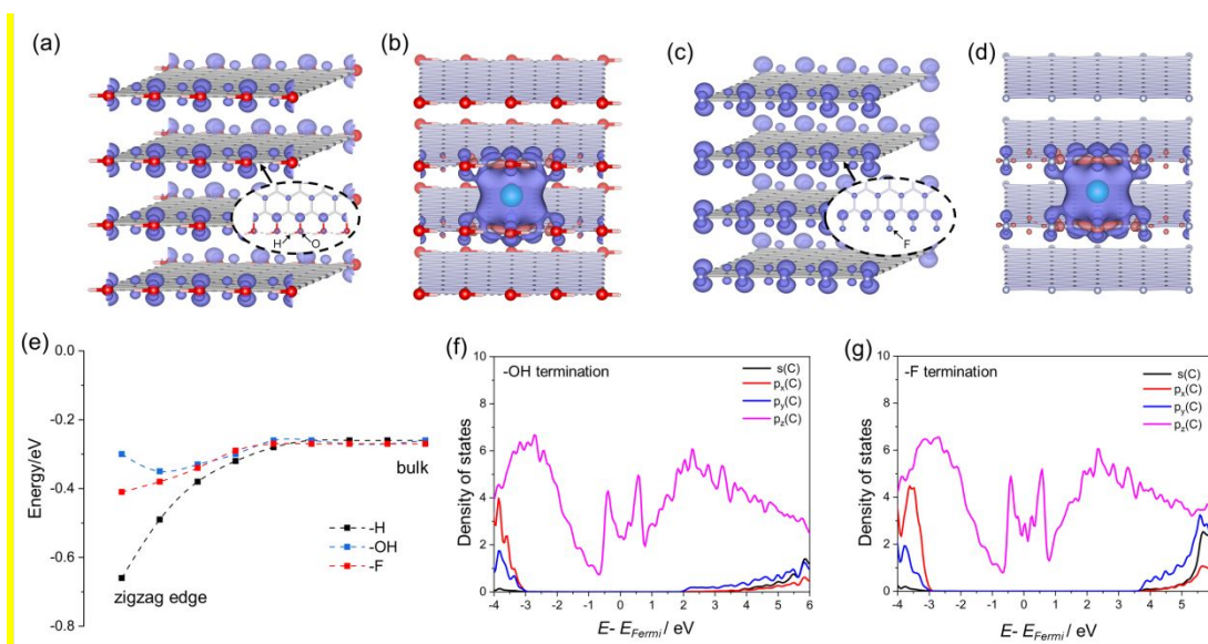
Figure S5. (a) shows the spin density accumulation on the edged carbon in OH-terminated zigzag-edged graphite. The inserted graph shows the top view of the basal plane of the graphite edge. The iso-surface value is 0.003 \text{ eV}/\text{\AA}^3 . (b) depicts the charge density difference of Li adsorption at the edge site in zigzag-edged graphite. (c) shows the spin density in F-terminated zigzag-edged graphite. The inserted graph shows the top view of the basal plane of graphite edge. The iso-surface value is 0.0015 \text{ eV}/\text{\AA}^3 . (d) is the charge density difference of Li adsorption at the edged site in F-terminated graphite. The iso-surface value is 0.001 \text{ eV}/\text{\AA}^3 . (e) shows Li adsorption energy change from the edged site to the bulk site in zigzag-edged graphite with different terminations on edged carbons. (f) and (g) are the local density of states (LDOSs) of edged carbons in OH-terminated and F-terminated zigzag-edged graphite.
