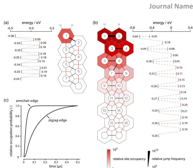
Figure 3. Li diffusion at (a) armchair-edged and (b) zigzag-edged graphite. Colored hexagons indicate site occupancy relative to bulk and the width of the lines connecting sites indicates jump frequency; (c) probability for Li to occupy a site approximately 20 Å below the surface relative to the steady-state value after being introduced at time zero at the edge.
