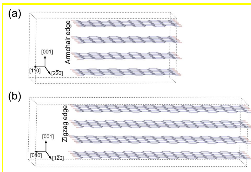
Figure S2. Periodic systems of armchair-edged and zigzag-edged graphite; (a) structure of hydrogen-terminated armchair-edged graphite ( a = 13.76 \text{ \AA} , b = 8.53 \text{ \AA} , c = 27.25 \text{ \AA} ; \alpha = \beta = \gamma = 90^\circ ); (b) hydrogen-terminated zigzag-edged graphite ( a = 13.76 \text{ \AA} , b = 9.86 \text{ \AA} , c = 46.98 \text{ \AA} ; \alpha = \beta = \gamma = 90^\circ ).
