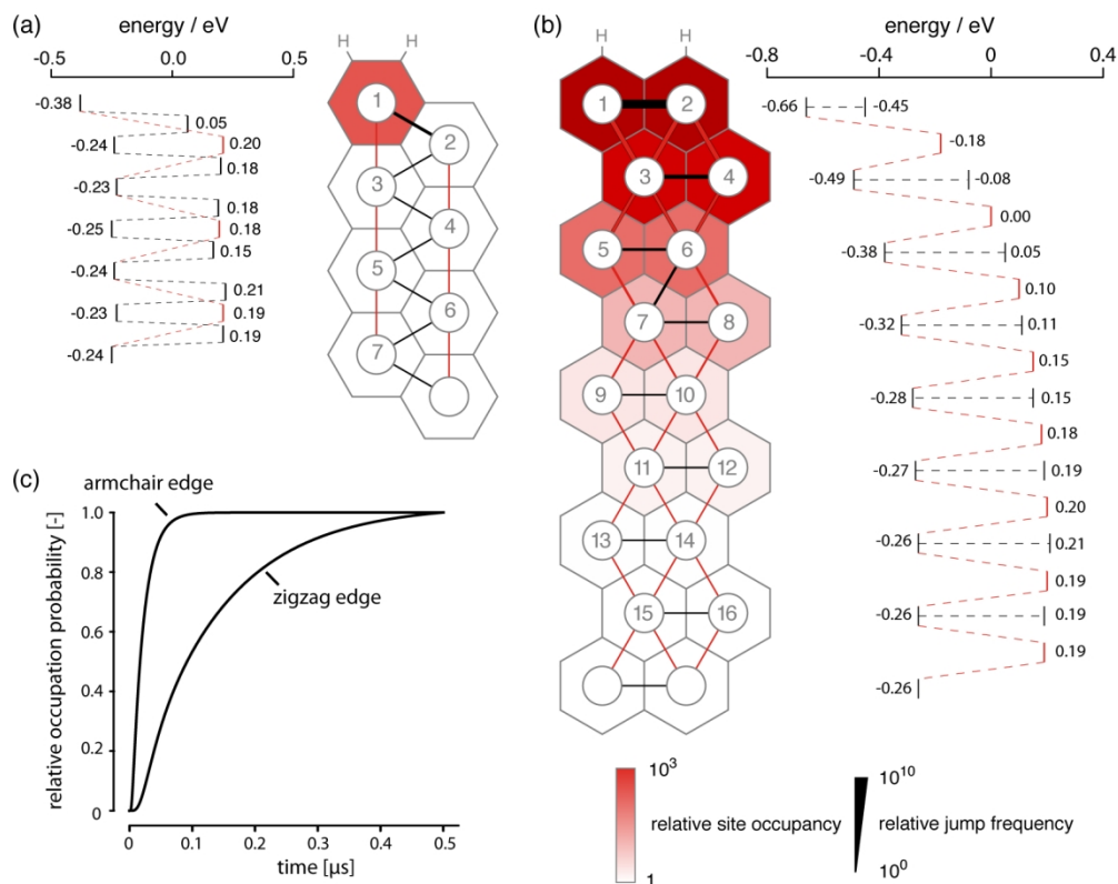
Li diffusion at (a) armchair-edged and (b) zigzag-edged graphite. Colored hexagons indicate site occupancy relative to bulk and the width of the lines connecting sites indicates jump frequency; (c) probability for Li to occupy a site approximately 20 Å below the surface relative to the steady-state value after being introduced at time zero at the edge.
