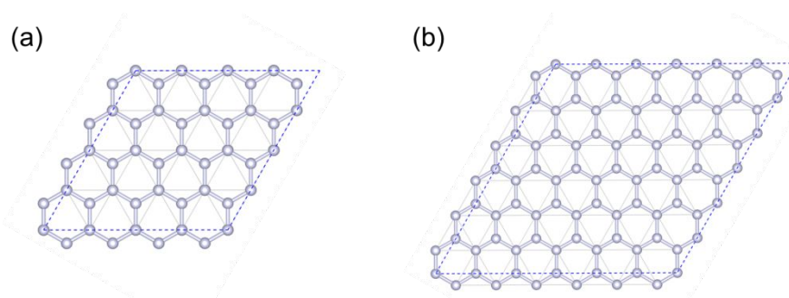
Figure S9. Structures of two graphite bulk with four graphene layers. (a) Bulk 1 ( a=b=9.86 Å, c=13.76 Å) has 128 C atoms. (b) bulk 2 ( a=b=14.78 Å, c=13.76 Å) contains 288 C atoms.
