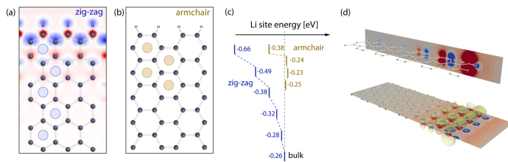
Geometrical structures of graphite edges for zigzag-edged graphite (a) and armchair-edged graphite (b). (c) is the profile of Li adsorption energies as a function of distance from the edge towards the bulk of graphite. (d) illustrates the spin densities in zigzag-edged graphite. The iso-surface value is 0.0002 \text{ e}/\text{\AA}^3 .
