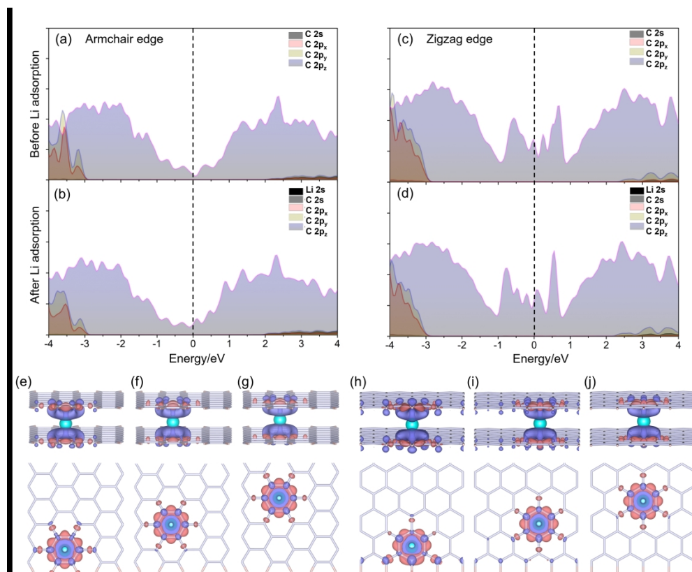
Local density of states (LDOSs) and charge difference of Li adsorption at armchair and zigzag edges. (a) and (b) are LDOSs of edge carbons at armchair edges before and after Li adsorption. LDOSs are projected on the first carbon hexagons at the armchair and zigzag edges. (e) ~ (g) and (h) ~ (j) are charge differences of Li adsorption at the edge site, sub-surface site and the bulk site relative to pristine graphite in armchair-edged and zigzag-edged systems, respectively. The iso-surface value is 0.001 \text{ e}/\text{\AA}^3 .
