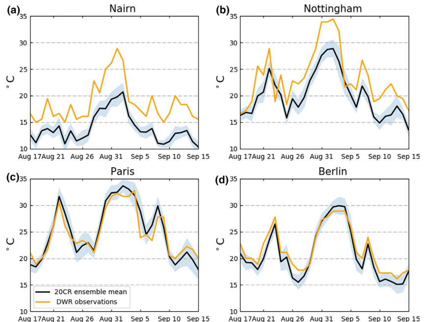
FIGURE 14 Observed DWR T_{\max} (orange line) and ensemble mean 20CRv3 2m T_{\max} (black line) with the ensemble spread (blue shading) at (a) Nairn, (b) Nottingham, (c) Paris and (d) Berlin. Units are ^{\circ}\text{C}
