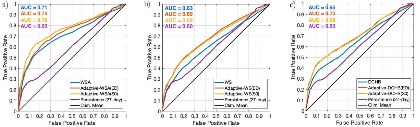
Figure 6. Receiver operator characteristic curves plotting the true positive rate (TPR) against the false positive rate (TPR) for a range of event thresholds for different models of the ambient solar wind including the WSA model, WS model, and the DCHB model (a)–(c), together with the 27-day persistence model (violet line) and the climatological mean (black line). The area under the curve (AUC) on the left hand corner is a summary variable of how well the model can predict the ambient solar wind.
