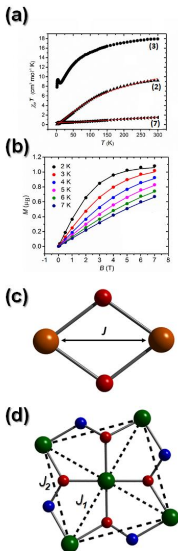
Figure 10 (a) Overlay \chi_M T versus T plots for polycrystalline sample of 2, 3, and 7 taken in the T = 300-2 K temperature range in an applied field, B , of 0.1 T for 2 and 3, and 0.5 T for 7. (b) Magnetisation ( M/\mu_B ) vs. B (T) data obtained from a polycrystalline sample of 7 measured in the 2-7 K temperature range and 0-7 T magnetic field range. (c and d) The exchange coupling schemes used to fit the data in 2 (c) and 7 (d). For 2; \hat{H} = -2J(\hat{S}_1 \cdot \hat{S}_2) and for 7; \hat{H} = -2J_1(\hat{S}_1 \cdot \hat{S}_5 + \hat{S}_2 \cdot \hat{S}_5 + \hat{S}_3 \cdot \hat{S}_5 + \hat{S}_4 \cdot \hat{S}_5) - 2J_2(\hat{S}_1 \cdot \hat{S}_2 + \hat{S}_2 \cdot \hat{S}_3 + \hat{S}_3 \cdot \hat{S}_4 + \hat{S}_4 \cdot \hat{S}_1) . The solid lines represent a simultaneous best-fit of the experimental susceptibility and magnetisation data as described in the main text. Colour code as described earlier in the text.
