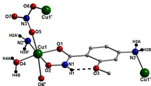
Figure 4 The asymmetric unit in \{[\text{Cu}(\text{II})(\text{L}_2\text{H})(\text{H}_2\text{O})(\text{NO}_3)] \cdot \text{H}_2\text{O}\}_n ( 4 ) along with the connector atoms (N2', O6', Cu1' and Cu1'') that propagate the 2D extended network in 4 . The majority of H atoms and the water of crystallisation have been omitted for clarity. Intramolecular H-bond represented as a dashed line (N1(H1)···O3 = 2.03 Å).
