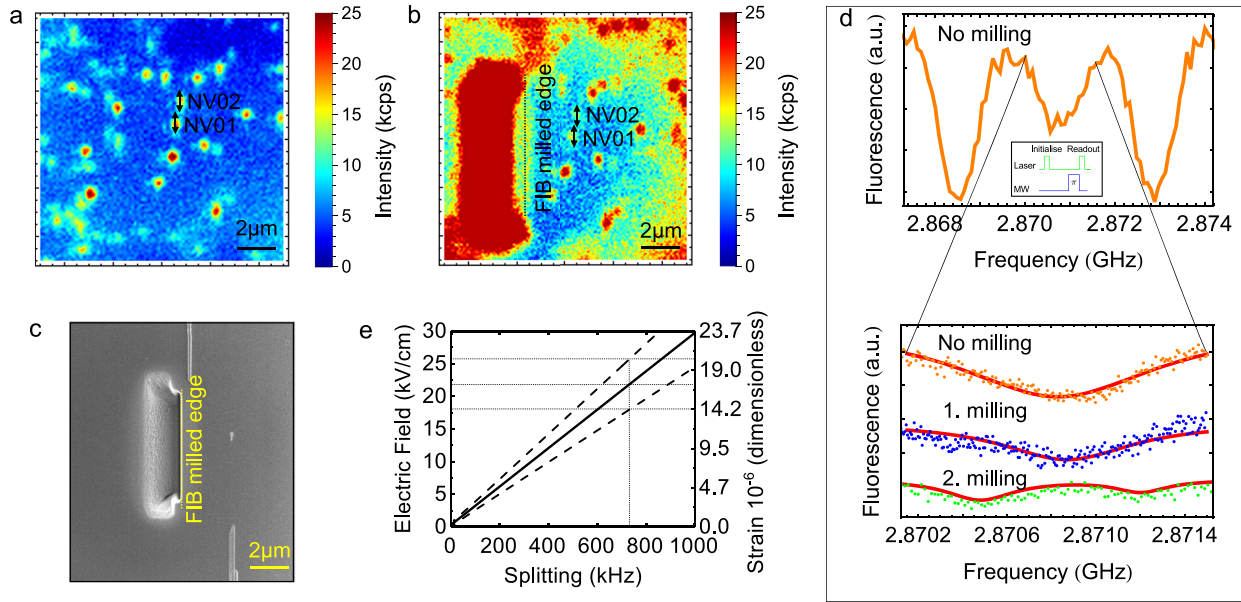
Fig. 1 NV centres near FIB milled interface. a, b Confocal image in the focal plane of NV01 and NV02 without and with focused ion beam milled edge at a 1.5 \mu\text{m} distance. c Corresponding ion-induced secondary electron image. The interface is milled to a depth of 8 \mu\text{m} and a width of 6 \mu\text{m} . d (top) Pulsed optically detected magnetic resonance (ODMR) example for NV02 in the case of no milling (data points are connected for clarity). Inset: Microwave \pi -pulse applied between two 532 nm laser pulses. The photoluminescence in the second laser pulse is detected, and plotted as a function of the microwave frequency. d (bottom) Pulsed optically detected magnetic resonance (ODMR) of NV02 |\pm 1, 0\rangle states. Indicated are no milling, 1. milling (1.5 \mu\text{m} ) and 2. milling (0.5 \mu\text{m} ) to the reference position of NV01. We cannot resolve any splitting in the unmilled case 0.60 \pm 0.05 MHz (single Lorentzian fit), a broadened Lorentzian fit for 1. milling to 0.80 \pm 0.05 MHz, and a splitting of 720 \pm 4 kHz for 2. milling (double Lorentzian). e The equivalent electric field (left axis) or strain (right axis) associated with a measured splitting. The dashed lines indicate the uncertainty.
