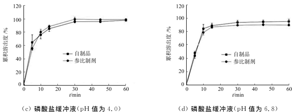
图3 自制品与原研制剂在不同溶出介质中的溶出曲线对比 Fig. 3 Comparison of dissolution curves of self-made products and innovator products in different dissolution media
