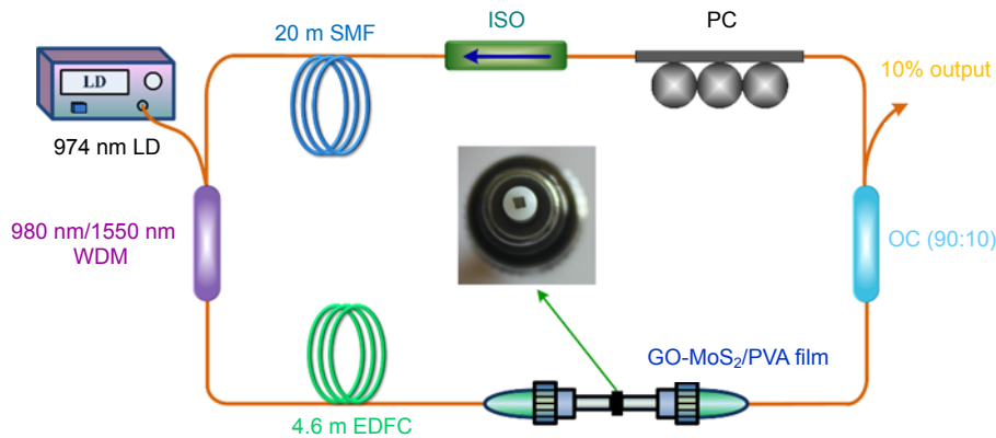
The structure of GO-MoS 2 -based EDFL
