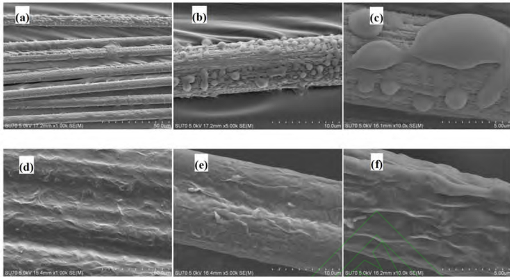
图 5 CF/E54-DDS(a,b,c)预浸料和 0.5%GO/CF/E54-DDS(d,e,f)预浸料的 SEM 图 Fig.5 SEM images of CF/E54-DDS prepreg (a,b,c) and 0.5%GO/CF/E54-DDS prepreg (d,e,f)
