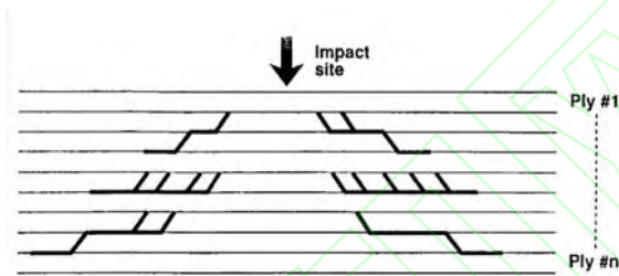
图 7 复合材料层合板冲击后锥形损伤示意图 [34] Fig.7 Schematic of cone of damage due to impact [34]
