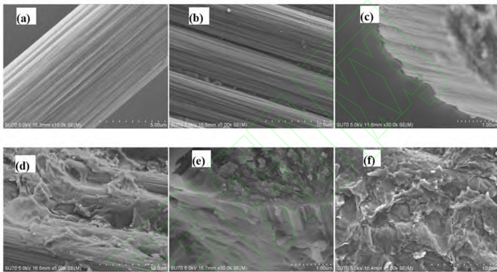
图 4 CF(a)、CF/E54-DDS(b,c)、0.5%GO/CF/E54-DDS(d,e)和 1.0%GO/CF/E54-DDS (f)的 SEM 图 Fig.4 SEM images of CF(a),CF/E54-DDS(b,c),0.5%GO/CF/E54-DDS(d,e) and 1.0%GO/CF/E54-DDS(f)
