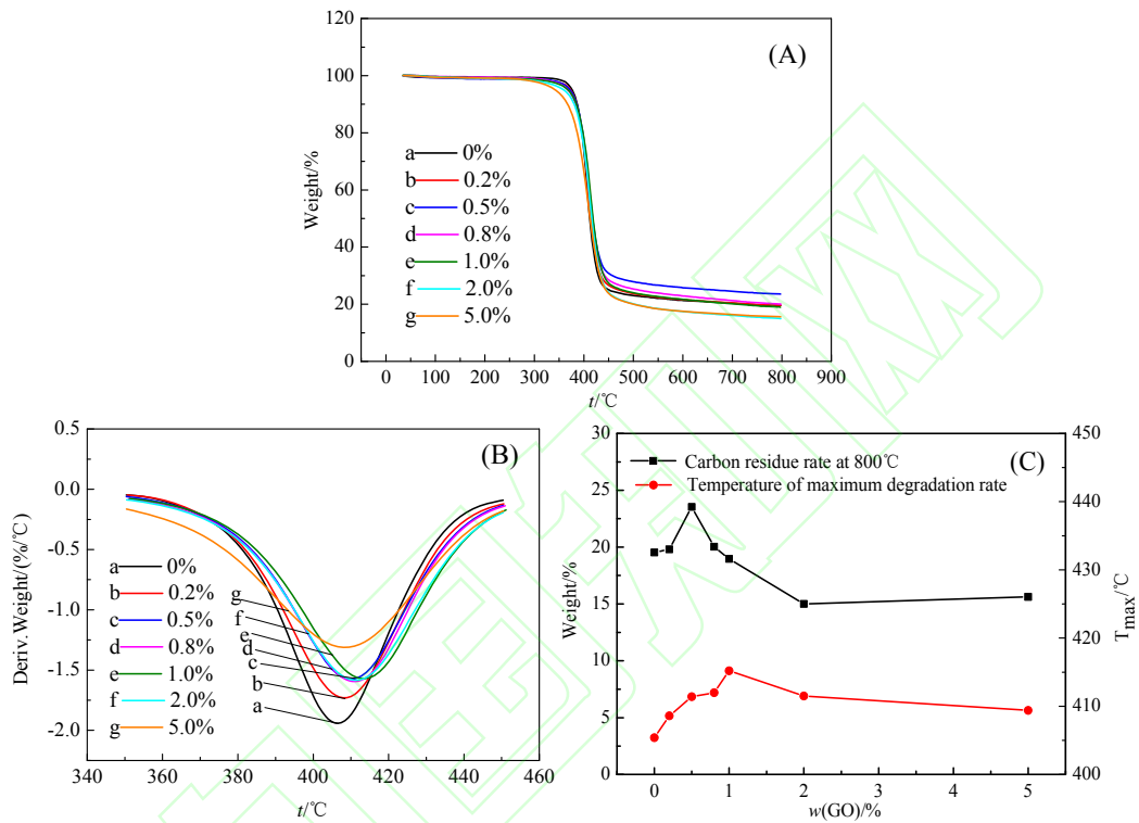
图 2 不同 GO 含量的 GO/E54-DDS 体系的热失重 TGA 曲线(A)、微商热重 DTG 曲线(B)、800℃的残碳率和最大失重速率温度 T_{max} (C) Fig.2 The TGA curves (A), DTG curves (B), carbon residue rate at 800℃ and temperature of maximum degradation rate (C) of GO/E54-DDS
