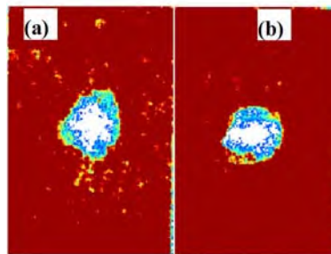
图 6 CF/E54-DDS(a)和 0.2%GO/CF/E54-DDS (b)冲击后 C 扫描图 Fig.6 The C scan result of CF/E54-DDS (a) and 0.2%GO/CF/E54-DDS(b) after impact
