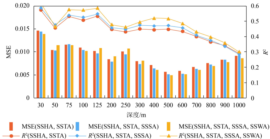
图 4 基于SVR模型的全球海洋15个不同深度层位STA估算结果的精度评价(评价指标采用均方差(MSE)和决定系数( R^2 )) Fig. 4 The performance measures comparison of 4-attributes (SSHA, SSTA, SSSA, SSWA), 3-attributes (SSHA, SSTA, SSSA) and 2-attributes (SSHA, SSTA) SVR for STA estimation at different depths (15 levels) based on MSE and R^2
