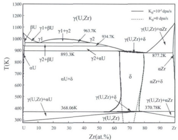
图 3 U-Zr 二元系辐照下的相图与热力学平衡相图的比较 [20] Fig. 3 Comparison of phase diagram under irradiation of U-Zr binary system with thermodynamic equilibrium phase diagram [20]
