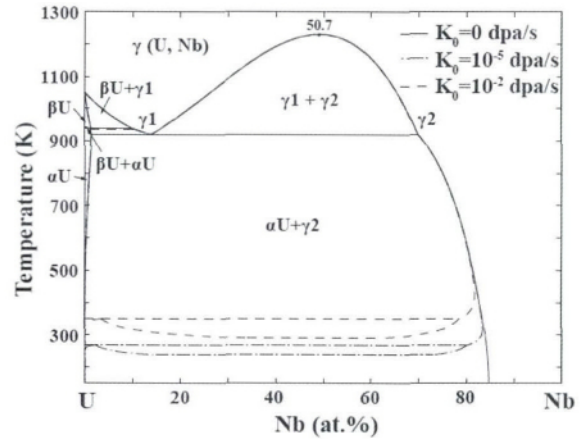
图 2 U-Nb 二元系辐照下的相图与热力学平衡相图的比较 [20] Fig. 2 Comparison of phase diagram under irradiation of U-Nb binary system with thermodynamic equilibrium phase diagram [20]
