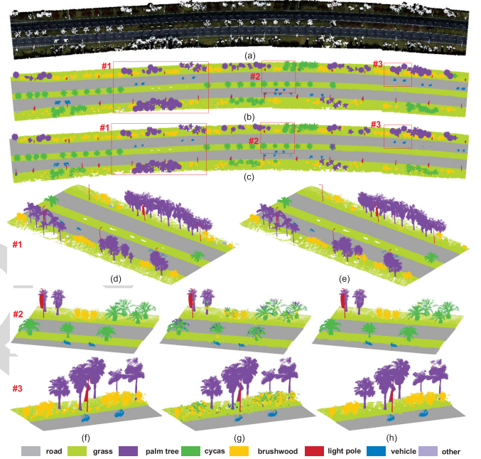
Fig. 7. Qualitative labeling results on a part of data set I. (a) Colorized point clouds. (b) Ground truth. (c) Semantic labeling results. (d) and (f) Close-up views of the ground truth in areas #1, #2, and #3. (g) Close-up views of the initial labeling results obtained by applying pairwise CRF model in areas #2 and #3. (e) and (h) Close-up views of the refined results obtained by incorporating regional label costs in areas #1, #2, and #3.
