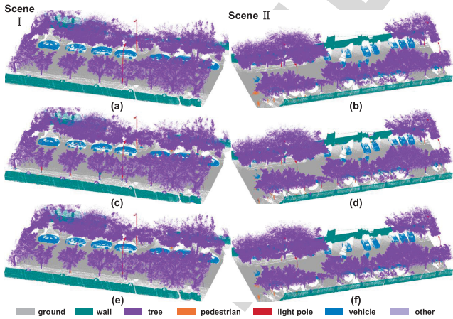
Fig. 8. Qualitative labeling results on two scenes in data set II. (a) and (b) Ground truth. (c) and (d) Initial labeling results. (e) and (f) Refined labeling results.
