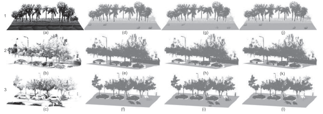
Fig. 13. Comparative labeling results on different scenes. (a)–(c) Colorized point clouds. (d)–(f) Ground truth. (g) and (h) Labeling results by applying 3D-PMG+MRF. (i) Labeling results by applying M3N. (j)–(l) Labeling results by applying our AL-Pairwise+LabelCosts.
