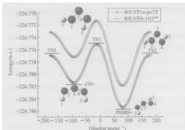
Fig.1 Potential energy curves of HOOOH by scanning dihedral angle
