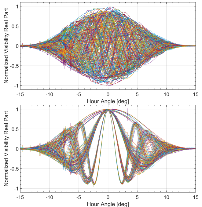
Figure 4. Real part of the complex visibilities corresponding to the transit of Cas A before (top panel) and after (bottom panel) calibration. Only the central channel at 407.6875 MHz is shown. Fringes show the main peak at transit ( \omega = 0^\circ ) where they are phased, i.e. where the geometrical delay is compensated. Each colour corresponds to one of the 276 independent baselines. Fringe spacings are proportional to baseline lengths, therefore redundant visibilities appear grouped in subsets that have similar fringe frequencies.
