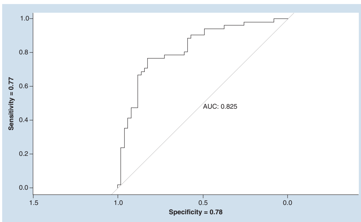
Figure 4. Receiving operating characteristic for horizontal saccades (fixation # and saccadic velocity to accuracy ratio) – no-traumatic brain injury versus traumatic brain injury.
