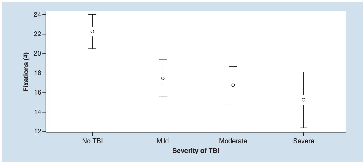
Figure 1. Mean values of fixation (#) at each level of traumatic brain injury severity, with 95% CI. For fixation (#) metrics – a higher value is better.
