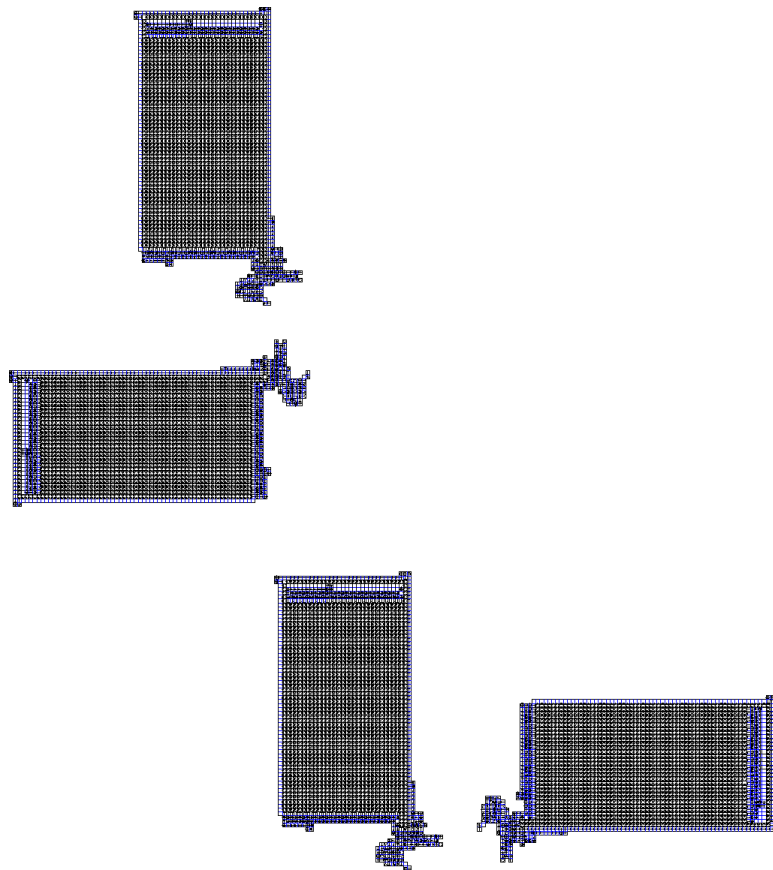
Fig. 12. SRMs after two generations
