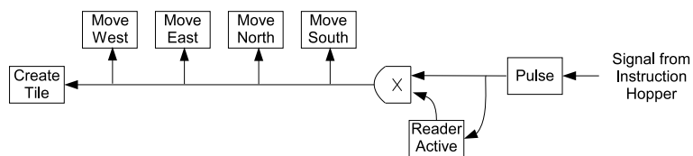
Fig. 6. The arrangement of the instruction tape.
