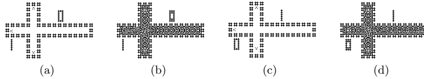
Fig. 7. NOT gate implementation for input '1' (a,b) and input '0' (c,d). This way (a) and (c) display initial configurations, (b) and (d) display final configurations.
