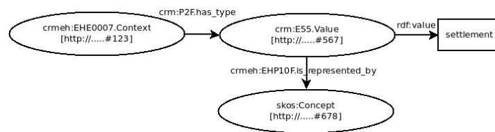
Fig. 1: A Semantic Annotation example containing a terminological and an ontological reference. The textual value of the annotation is “settlement” which is defined as an instance of the CRM-EH class EHE0007.Context. The value is linked (is_represented_by) a SKOS definition.
