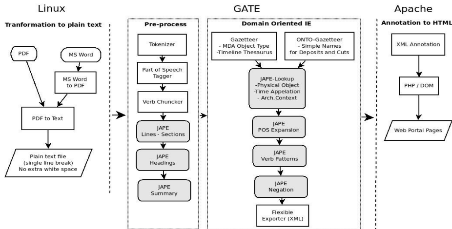
Fig. 2: The Information Extraction pipeline developed in GATE. Two separate exercises are shown here the Pre-processing and the Domain Oriented IE. Bespoke JAPE rules shown in Grey boxes, white boxes are used for GATE modules
