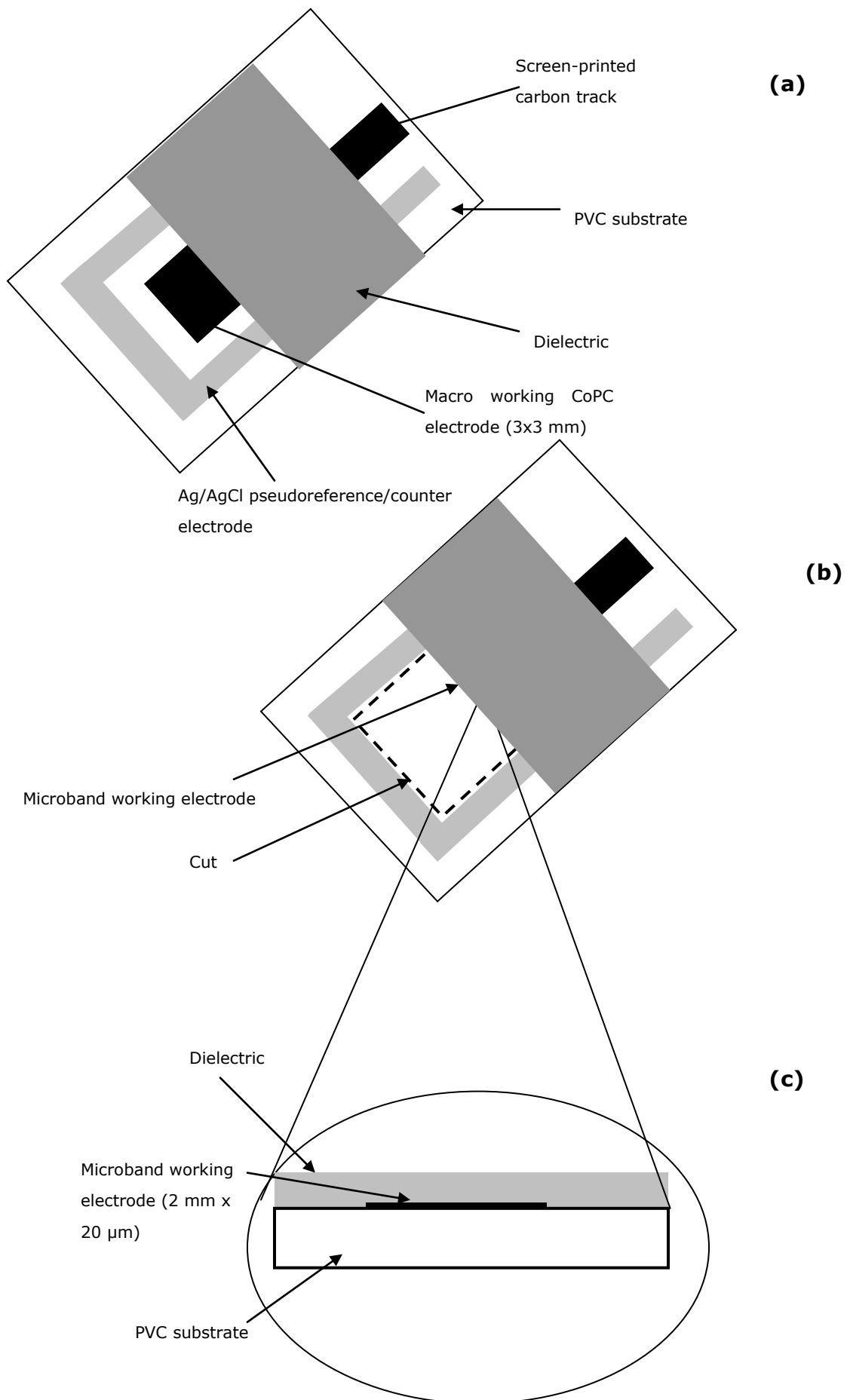
Figure 1 Schematic diagram demonstrating the method for the manufacture of microband SPCEs.
