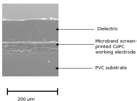
Figure 2. Scanning electron micrograph of a microband CoPC-SPCE.
