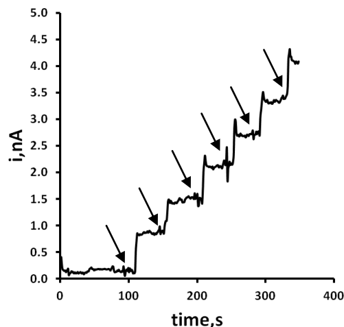
Figure 7. Chronoamperometric investigations of GSH at a microband CoPC-SPCE electrode in MEM dilute 1:1 with 0.2 M phosphate buffer solution, pH 7.4 at 37 °C. Arrows represent additions of 5 \mu L 102 mM GSH into 8 mL quiescent (stirred only to mix for 10 s).
