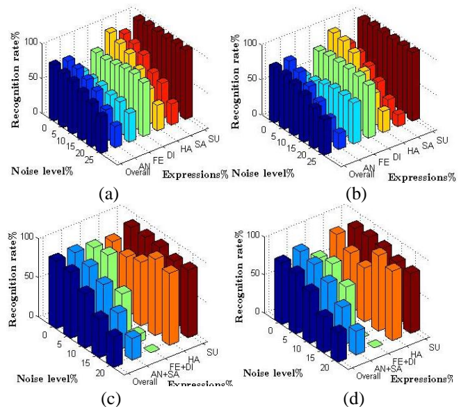
Figure 7. Recognition accuracy as function of the measurement noise level. (a) 3D data using supervised learning. (b) 2D data using supervised learning. (c) 3D data using unsupervised learning. (d) 2D data using unsupervised learning.
