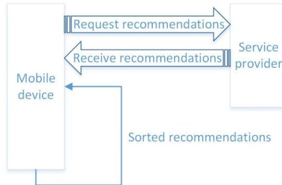
Figure 3. Client-Server interaction
