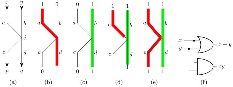
Figure 3: Gravity gate with two inputs and two outputs. (a) Scheme of the gate, the basic AND gate, i.e. p = xy and the basic OR gate, i.e. q = x + y . In subfigures (bcde) the development of gate is provided. (b) Root enters input channel x only, x = 1 and y = 0 . (c) Root enters input channel y only, x = 0 and y = 1 . (d) and (e) Roots enter both input channels x and y , x = 1 and y = 1 , at different time steps: (d) Time moment t = |b| + \sqrt{|a|} - 0.2 , where |a| and |b| are lengths of channels a and b . (e) final state. (f) Equivalent logic gates design, namely AND and OR gates. Coloured inputs symbolise channels occupied by roots. Red and green colour are only here to show how roots originated at different inputs interact.
