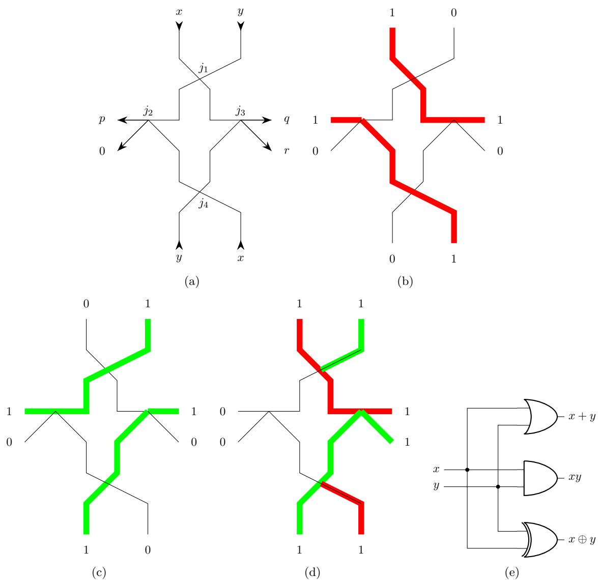
Figure 6: A half-adder made of two humidity gates. (a) Scheme of the circuit, p = x \oplus y , q = x + y , r = xy . (b) x = 1 and y = 0 . (c) x = 0 and y = 1 . (d) x = 1 and y = 1 . (e) Equivalent logic gates design.
