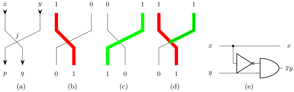
Figure 5: (a) Scheme of humidity gate with two inputs x and y and two outputs p and q : p = \bar{x}y and q = x . (b) x = 1 and y = 0 . (c) x = 0 and y = 1 . (d) x = 1 and y = 1 . (e) Equivalent logic scheme.
