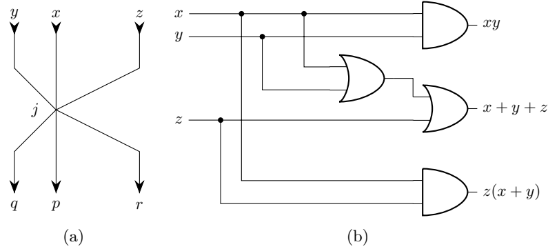
Figure 4: (a) Three-inputs-three-outputs gravity gate: q = xy and p = x + y + z and r = z(x + y) and (b) its equivalent logical scheme.
