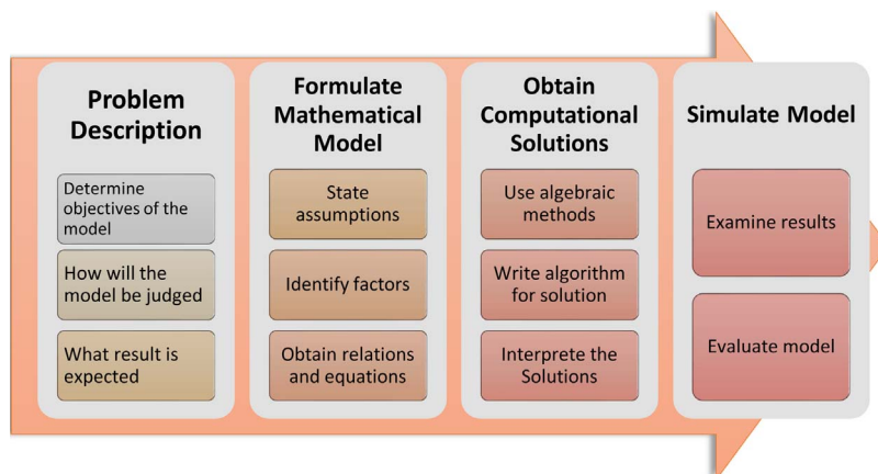
Fig. 2. Mathematical Modelling Process.
