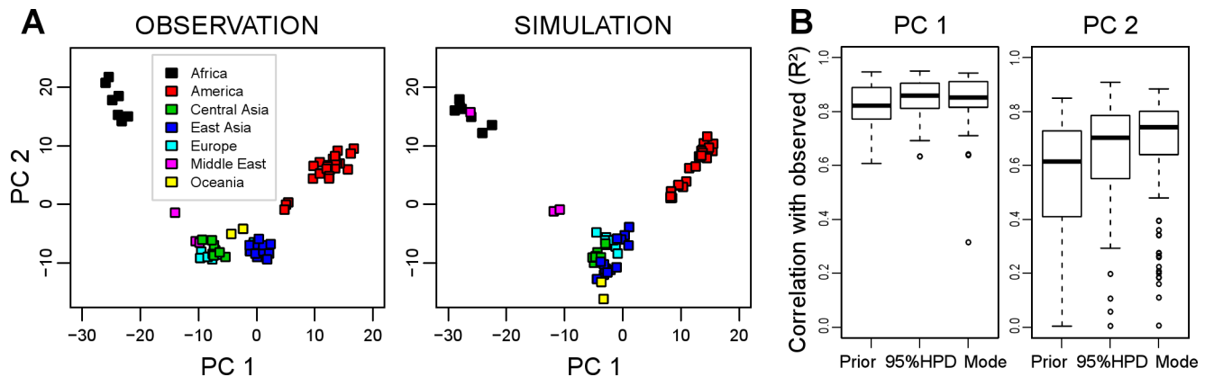
Fig 3. PCA results in real observation and simulations. A, Comparison of PCA applied to the empirical data (left) and one selected simulation (right). The first (PC 1) and second (PC 2) principal components are represented here, where each point represents one of the analyzed populations, grouped by continents. B, Boxplots of the correlation values between the first two principal components in observations and simulations based on the prior distribution (“Prior”), 95% higher posterior density distribution (“95%HPD”), and on the point estimates (“Mode”).
