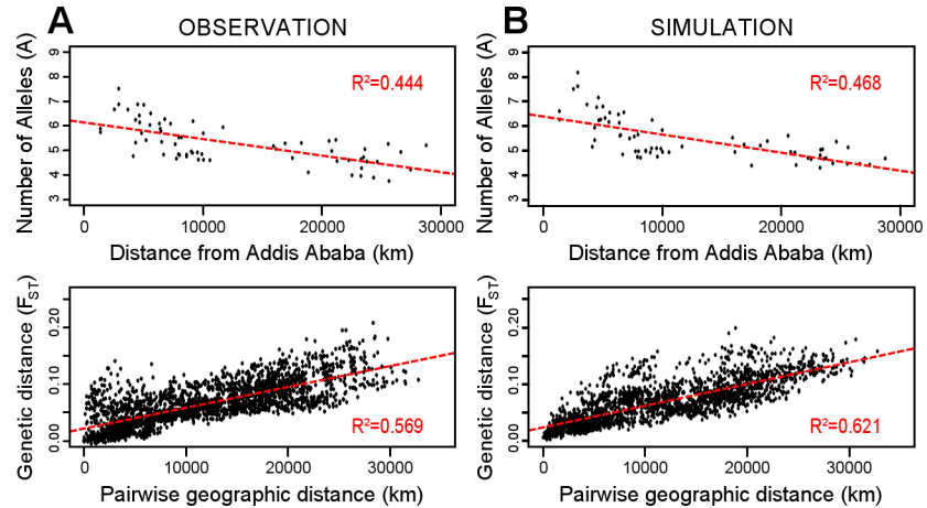
Fig 1. Comparison of the patterns of isolation by distance generated with the empirical and simulated data. In A, the patterns obtained for the observed data; in B, the result of one of the simulations based on the point estimates. Each point represents a population (top) or a pairwise population comparison (bottom); the dashed lines represent the linear regressions of these points (whose R^2 values are informed).
