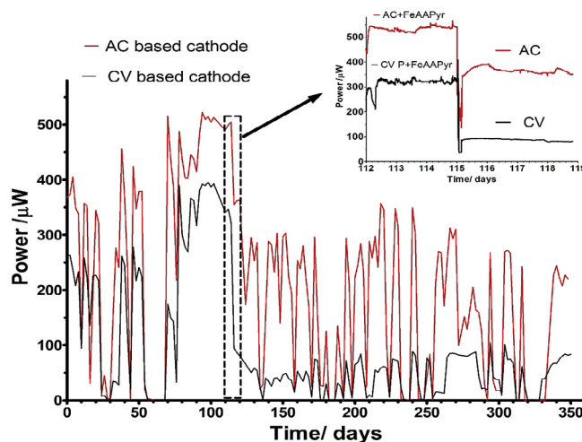
Fig. 4. Temporal power behaviour of the MFCs, over 350 days of operation. The MFCs (mean values of triplicated data) were fed with activated sludge wastewater supplemented with sodium acetate as the carbon energy source. The arrow indicates the cathode replacement from catalyst based to non-catalyst based material (inset).
