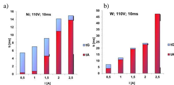
Fig. 12. Comparison of total discharge time ( t_i ) and portion of the glow duration ( t_G ) for nickel and tungsten as contact materials when interrupting inductive load DC (110V, 10ms) at different current value in air under normal pressure ( \sim 100 kPa)
