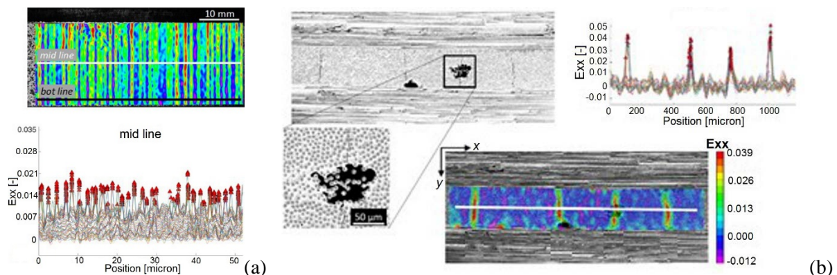
Figure 5. DIC-enhancement of the edge crack registration: (a) cracks identified as peaks on the strain profile; (b) cracks related to voids in 90^\circ plies [8].
