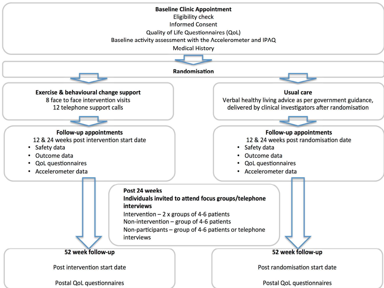
Figure 1 Consort diagram.
