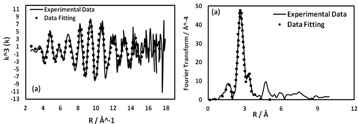
Figure 2. The ex-situ EXAFS Chi data and Fourier transforms and their fitting results for catalyst sample 15Pdanc25r36, phase corrected. The data were collected at ambient room temperature in air. The solid lines represent the experimental data, and the dotted symbols represent the fitted data.
