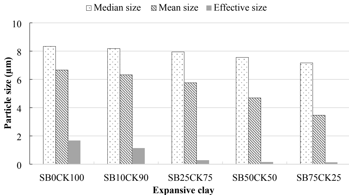
Fig. 6. Expansive clay particle size statistics.
