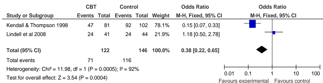
Figure 3: Forest plot of return to work studies
