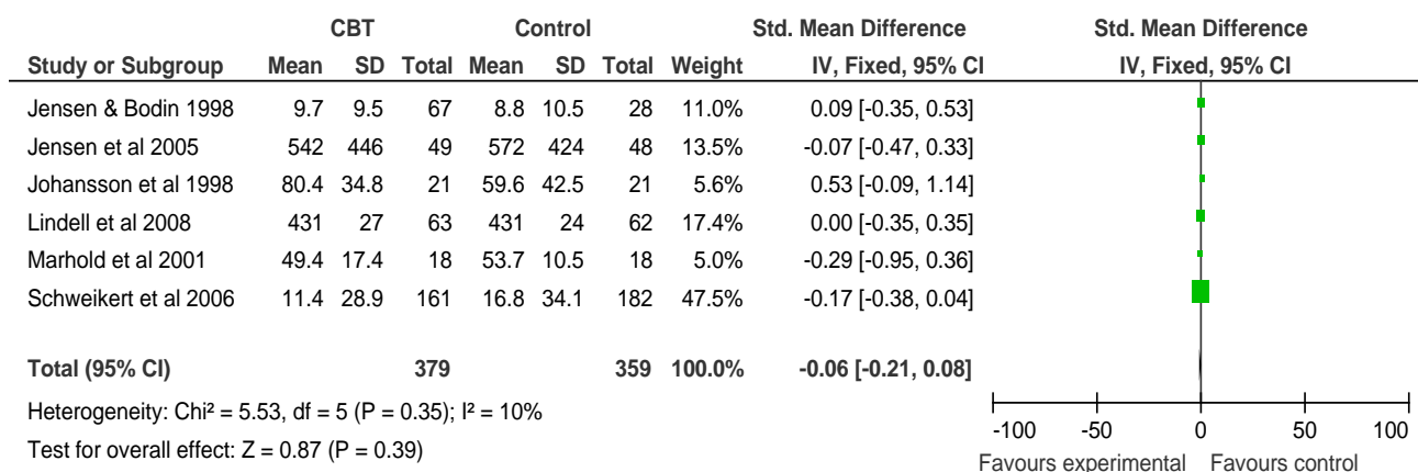
Figure 4: Forest plot of studies with sickness absence outcomes
