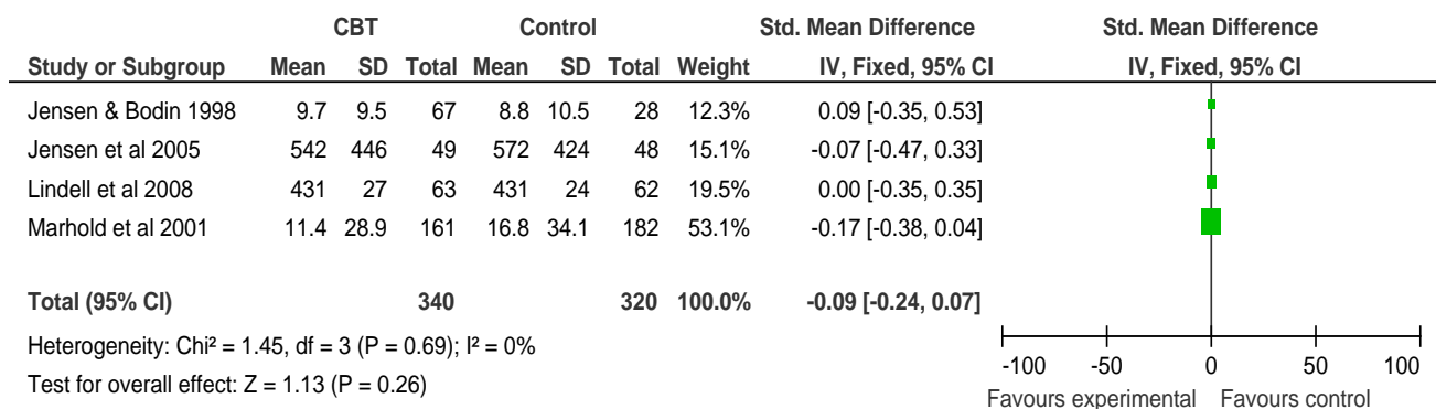
Figure 5: Meta-analysis of Swedish studies with sickness absence outcomes
