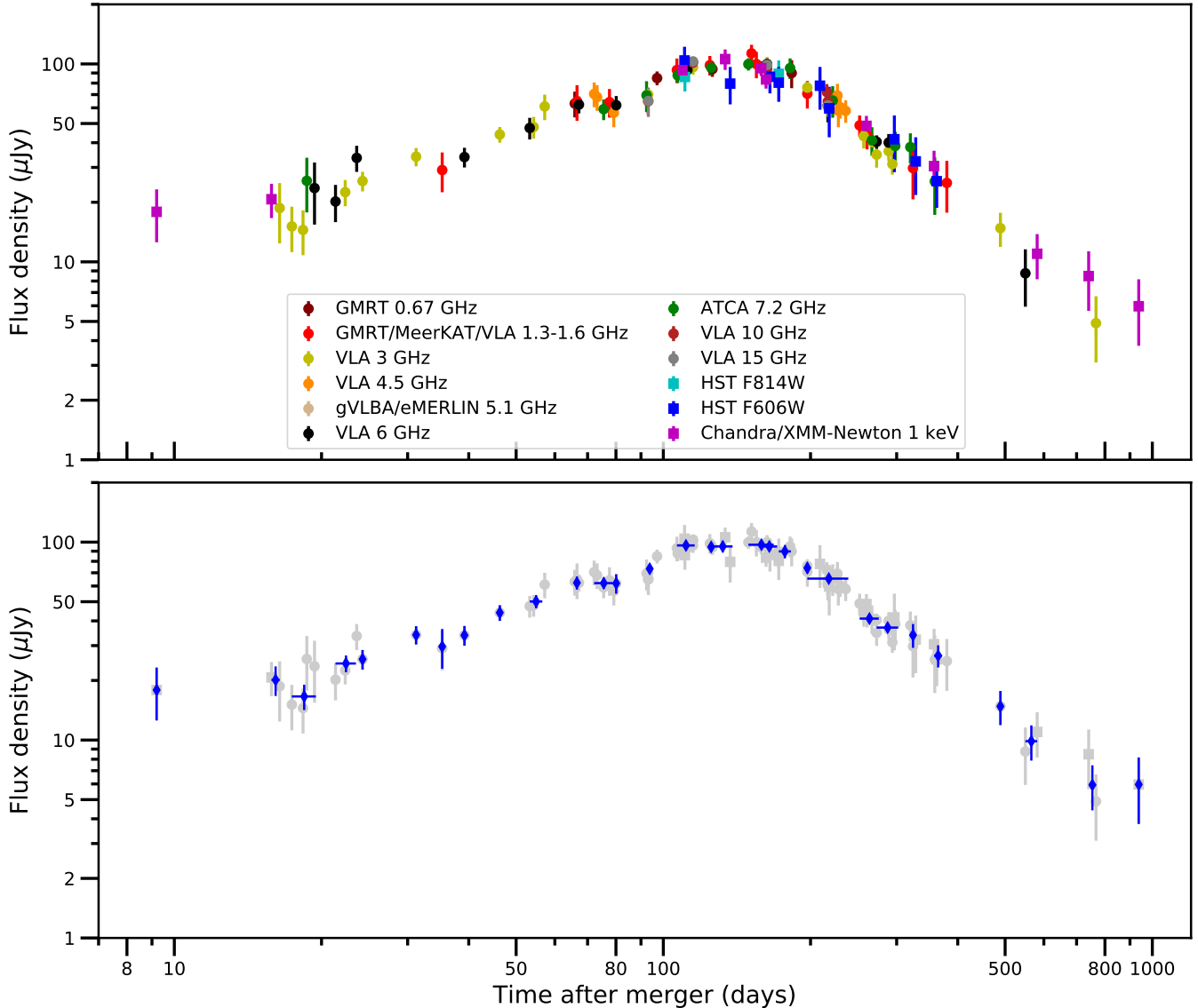
Figure 1. Upper panel: The panchromatic (radio, optical and X-ray) afterglow light curve of GW170817, color coded according to the observing frequency, up to 940 days post-merger (all data points have 1\sigma errorbars as presented in Table 1; upper limits are not shown here) using the uniform dataset presented in this work. The light curve is scaled to 3 GHz using the best-fit spectral index ( -0.569 ) derived from the MCMC power-law fitting (see §3). Lower panel: The averaged (using moving average; \Delta t/t = 1/17 where \Delta t is the width of the kernel and t is the time after merger) light curve (blue data points) shows a general trend consistent with power-law rise and decline. In grey are the same data points as shown in the upper panel.
