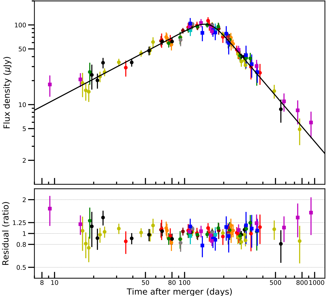
Figure 2. Broken power-law fit (using MCMC; best-fit shown as a black curve in the upper panel and residual shown in the lower panel) to the afterglow light curve. The corner plot for the MCMC analysis is shown in Figure 3. The light curve is scaled to 3 GHz using the best-fit spectral index ( -0.569 ) derived from the MCMC analysis. Color coding is the same as in Figure 1. The light curve rises as t^{0.86 \pm 0.04} and declines as t^{-1.90 \pm 0.12} . The light curve peak occurs at 155 \pm 4 days post-merger. The lack of any substantial outlier data points indicates that the afterglow is optically thin throughout its evolution, with the synchrotron self-absorption frequency lying below the radio band and cooling frequency lying above the soft X-ray band. See §3 for details.
