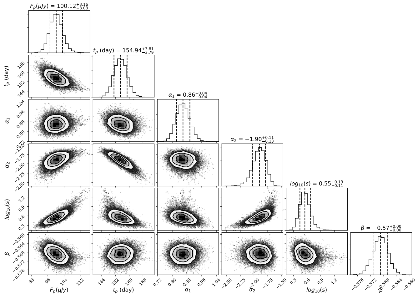
Figure 3. Corner plot for broken power-law fit to the light curve presented in Figure 2. Here, \beta is the spectral index, F_p is the flux density at 3 GHz at light curve peak, t_p is the light curve peak time, and \alpha_1 and \alpha_2 are the power-law rise and decay slopes, respectively.
