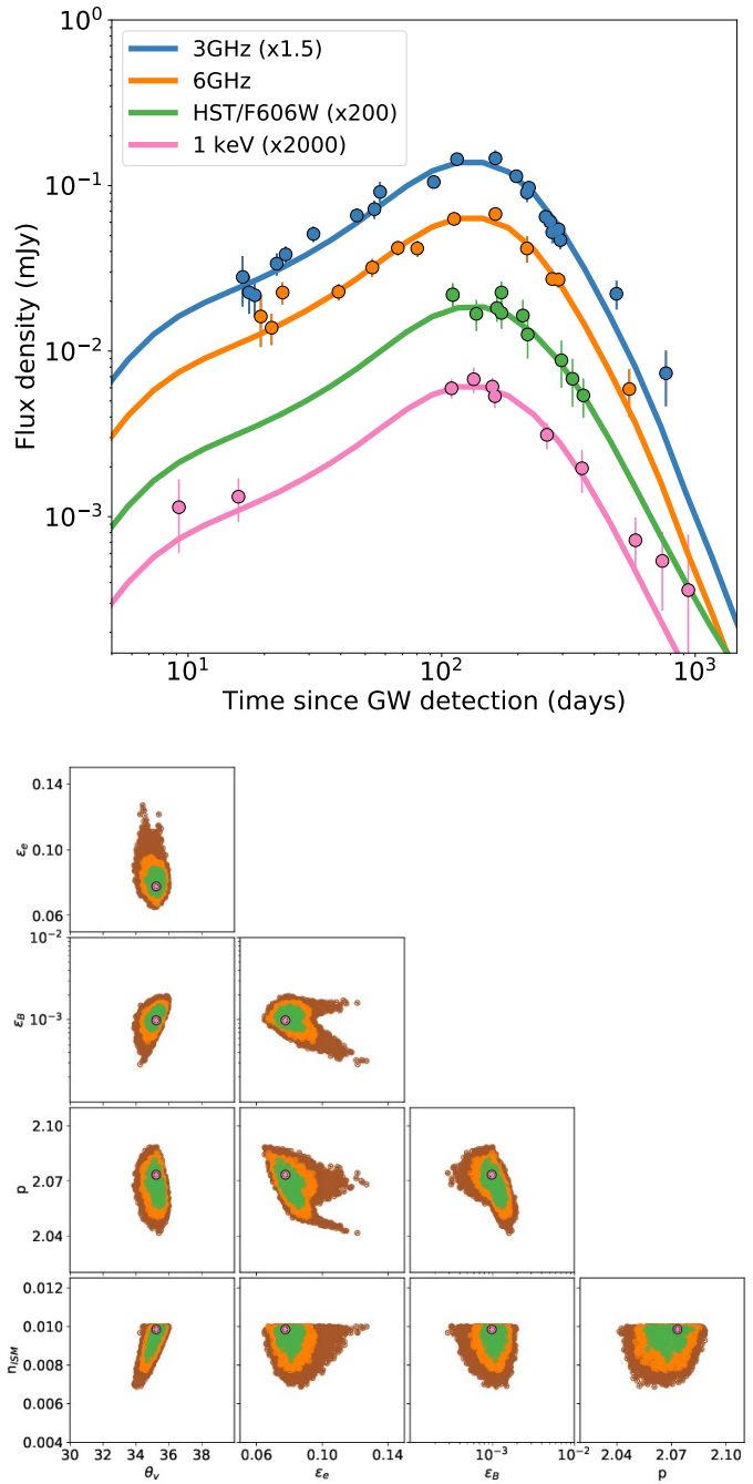
Figure 5. Upper panel: Structured jet model fit to the afterglow light curve using the forward-shock model from Lazzati et al. (2018). The best-fit model from the MCMC analysis is shown and color coding is according to the observing frequency. Only a subset of the observational data is plotted in this figure. Lower panel: Corner plot for the structured jet model. The pink dot shows the best-fit value for each parameter, and green indicates the 67% confidence interval. See §5.1 for details.
