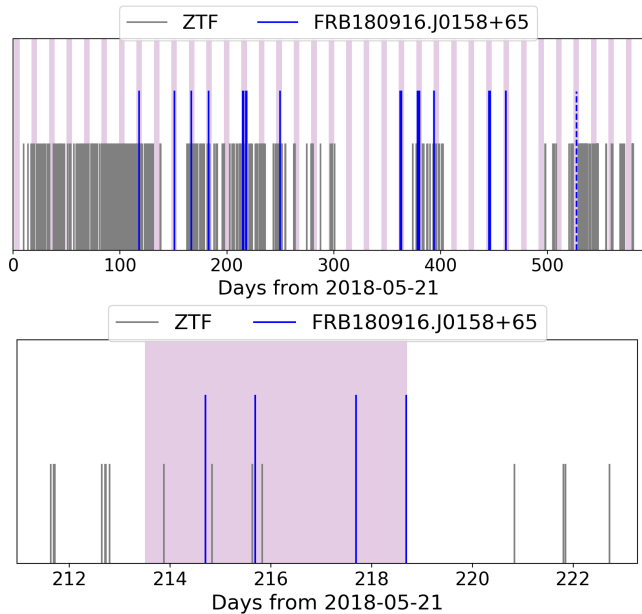
Figure 2. Top – ZTF observations (grey lines) and FRB 180916.J0158+65 detections (blue lines; CHIME/FRB Collaboration et al. 2019b; The CHIME/FRB Collaboration et al. 2020; Marcote et al. 2020). Purple bands indicate regions of high FRB activity, determined using a period of 16.35 d and a time window of 2 \times 2.6 \text{ d} around the estimated activity peak (The CHIME/FRB Collaboration et al. 2020). Dotted lines (un-resolved) indicate 2 FRBs detected on 2019 October 30, after a CHIME instrument upgrade. Bottom – Same as the top panel, zoomed in a region of the plot where 4 bursts were detected, two of which minutes to hours from ZTF observations.
