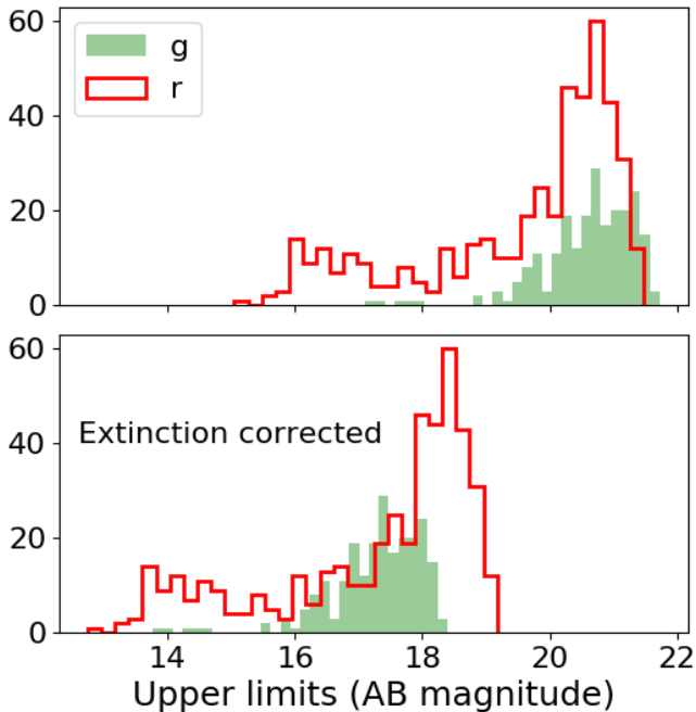
Figure 3. Top – Distribution of 3\sigma upper limits (apparent magnitude in AB system) on 683 ZTF images. Bottom – the same distribution is shown after correcting for Galactic extinction along the line of sight using the (Schlafly & Finkbeiner 2011) dust maps.
