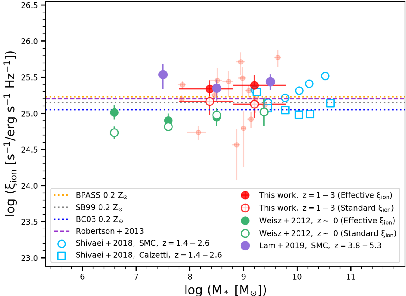
Figure 3. \log(\xi_{ion}) as a function of \log(M_*) . \log(\xi_{ion}) derived from the Standard stacking method are shown in red open circles and the Effective stacking method in red filled circles. The \log(\xi_{ion}) inferred from Effective method is \sim 0.2 dex larger than that of the Standard method. Green open and filled circles denote the local sample of Weisz et al. (2012) applying the Standard and Effective stacking methods respectively. Sky blue open squares and circles denote the MOSDEF sample (Shivaei et al. 2018) of higher stellar mass galaxies using Calzetti et al. (2000) and SMC Gordon et al. (2003) UV dust corrections respectively. Purple circles show the Lam et al. (2019) sample of faint ( L_{UV} < 0.2 L_* ) galaxies at higher redshifts ( z = 3.8 - 5.3 ). For a better comparison of samples with similar stacking methods, we use open markers to indicate the Standard stacking method and filled markers to indicate the Effective stacking method. The dashed line is the canonical value of 25.2 from Robertson et al. (2013). The local sample of Weisz et al. (2012) indicates lower \log(\xi_{ion}) compared to ours. High-redshift samples of Shivaei et al. (2018) and Lam et al. (2019) lie within the 1\sigma error bars of our two stacking methods. Orange, gray, and blue lines indicate the \log(\xi_{ion}) predicted by three different single stellar models, (BPASS model (Eldridge et al. 2017), Starburst99 (Leitherer et al. 2014), and BC03 (Bruzual & Charlot 2003)), assuming a constant star formation history and 0.2Z_{\odot} metallicity.
