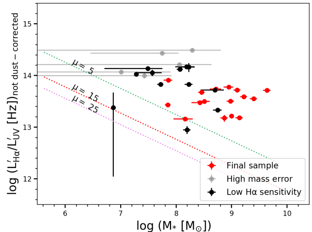
Figure 1. Not dust-corrected \log(L'_{H\alpha}/L'_{UV}) as a function of \log(M_*) derived from the observed L_{H\alpha} and L_{UV} . The gray points show galaxies with high mass errors. Black points indicate galaxies that could not be detected if they had the very low observed \log(L'_{H\alpha}/L'_{UV}) < 13.2 . The green, red and magenta diagonal dotted lines indicate the typical \log(L'_{H\alpha}/L'_{UV}) detection limit for three magnification factors of 5, 15 and 25 respectively, below which galaxies are intrinsically too faint to be detected through MOSFIRE. The remaining galaxies in red are free of any biases in our measurements.
