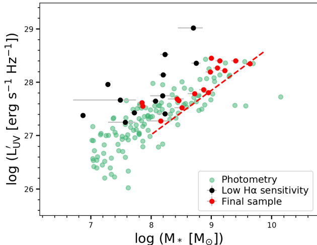
Figure 2. Not dust-corrected \log(L'_{UV}) - \log(M_*) relation of our lensed galaxies. Green points are the parent photometric sample with M_* above 10^7 M_\odot . The final spectroscopic \xi'_{ion} sample is shown in red. Black points are removed from the \xi'_{ion} sample due to biases discussed in Section 3.4. The galaxies in our final sample (red points) span a similar range in L'_{UV} at a given mass as the parent population, indicating that this sample is representative of low-mass galaxies at 1 < z < 3 . The red line denotes the lower edge of the \log(L'_{UV}) - \log(M_*) main sequence trend of the parent sample that is used to exclude galaxies with insufficient sensitivity (black points) from the \xi'_{ion} sample described in Section 3.5.
