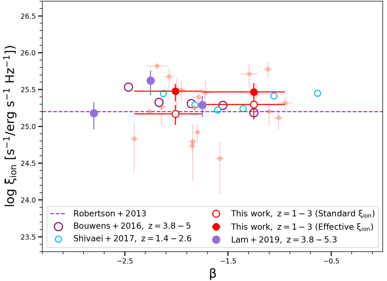
Figure 5. \log(\xi_{ion}) as a function of UV slope \beta . The symbols are the same as in Figure 4. No dependence of \log(\xi_{ion}) with \beta is seen in our sample.
