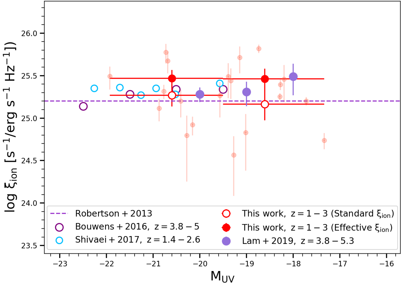
Figure 4. \log(\xi_{ion}) as a function of UV magnitude, M_{UV} . Small, light red circles denote individual galaxies in our sample. The large open and filled red circles show the \log(\xi_{ion}) derived from the Standard and Effective stacking methods, respectively. Sky blue circles show the stacks from Shivaiei et al. (2018) for more massive z \sim 2 galaxies and an SMC UV dust correction. Dark and light purple circles denote Bouwens et al. (2016) and Lam et al. (2019) samples at z \sim 4 - 5 respectively. Similar to Figure 3, for a better comparison of samples with similar stacking methods, we use open markers to indicate the Standard stacking method and filled markers to show the Effective method. Our values agree with other studies within 1\sigma significance when the same stacking method as ours are used. No significant dependence of \log(\xi_{ion}) with M_{UV} is found.
