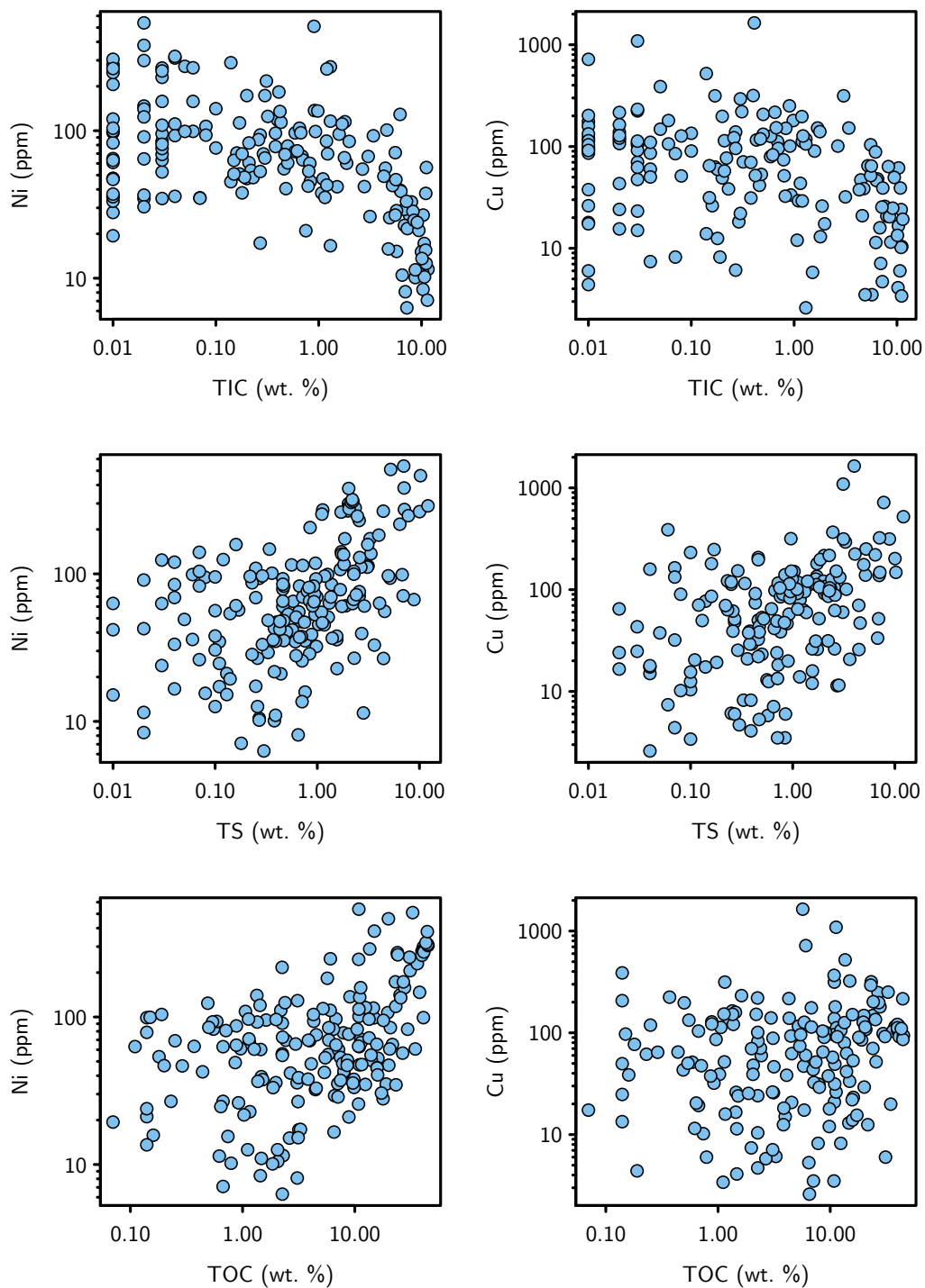
Figure S1. Ni and Cu concentrations versus total inorganic carbon (TIC), total sulfur (TS) and total organic carbon (TOC) in core 12AB (left) and core 13A (right).
