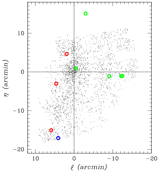
Figure 10. Spatial distribution of candidate ONC runaways. Background objects are the same as in Figure 3 but shown in tangential coordinates \xi , \eta . Runaways are divided in three parts: 1) confirmed by HST proper motions the likely Da Rio et al. (2012) photometric low-mass members of the ONC (red circles); 2) an additional candidate from HST proper motions (blue); 3) selected candidates from the Gaia DR 2 catalog (green). A nearest runaway to the Trapezium is the BN object, not detected by HST nor Gaia but also marked green.
