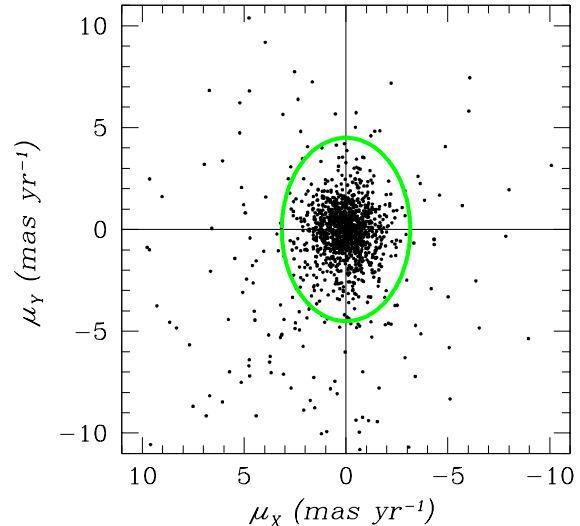
Figure 5. Vector-point diagram of sources shown in Figure 4. Green ellipse indicates the limit of selected proper motions used to calculate the internal velocity dispersion of the ONC.
