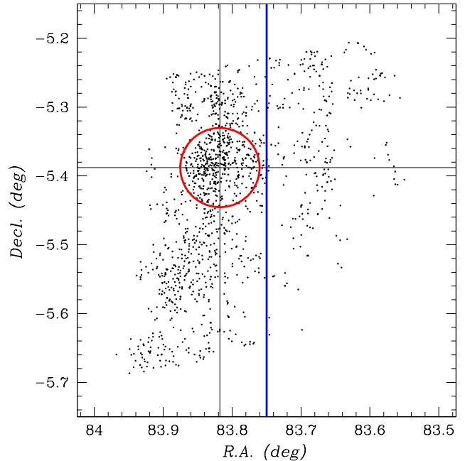
Figure 4. Spatial distribution of the selected 1379 sources with more reliable proper motions. Red circle: inner area of the ONC with a radius of 3'.45 centered on Trapezium; vertical blue line: cut-off at R.A. = 83^{\circ}75' separating the western sources with a possibly lower accuracy of proper motions.
