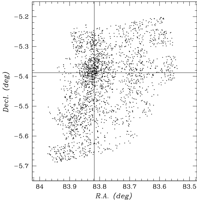
Figure 3. Spatial distribution of all sources with measured proper motions. Location of the Trapezium is marked by crosshairs.
