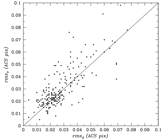
Figure 2. Distribution of rms errors from the least-squares transformations for all frame-tile, tile-strip, and strip-strip solutions. Nomenclature of these solutions is provided in Platais et al. (2015). The small number of common stars in several frame-tile solutions usually yields a high rms error.
