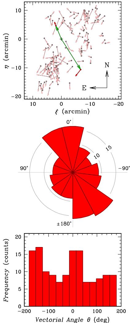
Figure 7. From a spatial map of tangential velocities of the ONC to one-dimensional histogram of vectorial angles. Upper panel: a spatial distribution of 141 fast-moving sources and their proper motions in the tangential plane with zero-point at the location of Trapezium, marked by a small cross. The length of arrows is proportional to the size of proper motions. Vectorial angle between the position vector and the arrow of a proper motion is a key parameter to identify potential runaways. Position vectors (in green) are drawn to the location of two sources: a Northern source has a very small vectorial angle \Theta = -2.3^\circ and is a likely runaway candidate, while a Southern source has \Theta = -71^\circ and is a passing-by field star. Middle panel: polar histogram of vectorial angles for all sources in the upper panel. The size of bins is 27.7^\circ and the upper bin is centered on \Theta = 0^\circ . The radial coordinate indicates the number of sources in each bin. Bottom panel: same as in the middle panel but transformed into the one-dimensional histogram of vectorial angles. Only the central bin at \Theta = 0^\circ contains likely runaways. The presence of other peaks is discussed in Section 3.2.1.
