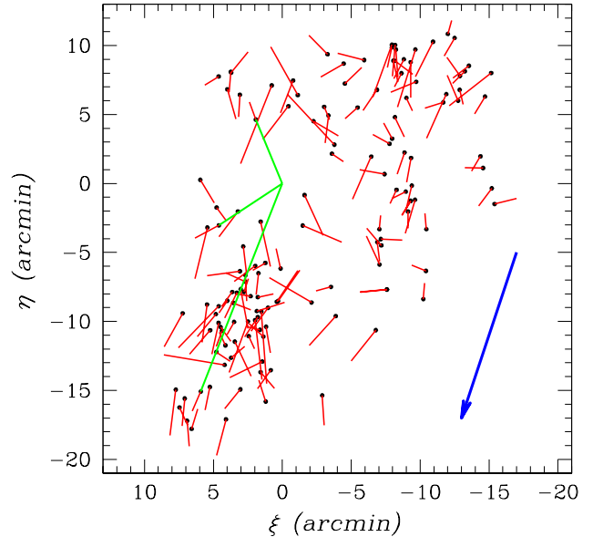
Figure 9. Spatial distribution of our faster-moving sources. Proper-motion vectors are shown by red line-segments at a scale of 5 \text{ mas yr}^{-1} per 1' . The total proper motions range from 5 to 30 \text{ mas yr}^{-1} . Three green lines with their origin at the Trapezium indicate new low-mass candidate runaways from our HST Treasury programs of the ONC. Blue arrow shows the dominant direction of Orion's A faster-moving young stellar objects.
