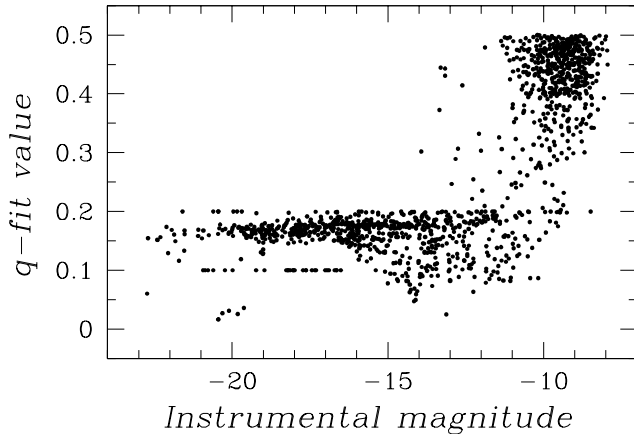
Figure 1. Distribution of the quality parameter qfit for sources measured in the central ONC image jcol35inq . Only a small fraction of detections with instrumental magnitudes brighter than -16 are stars and other sources.
