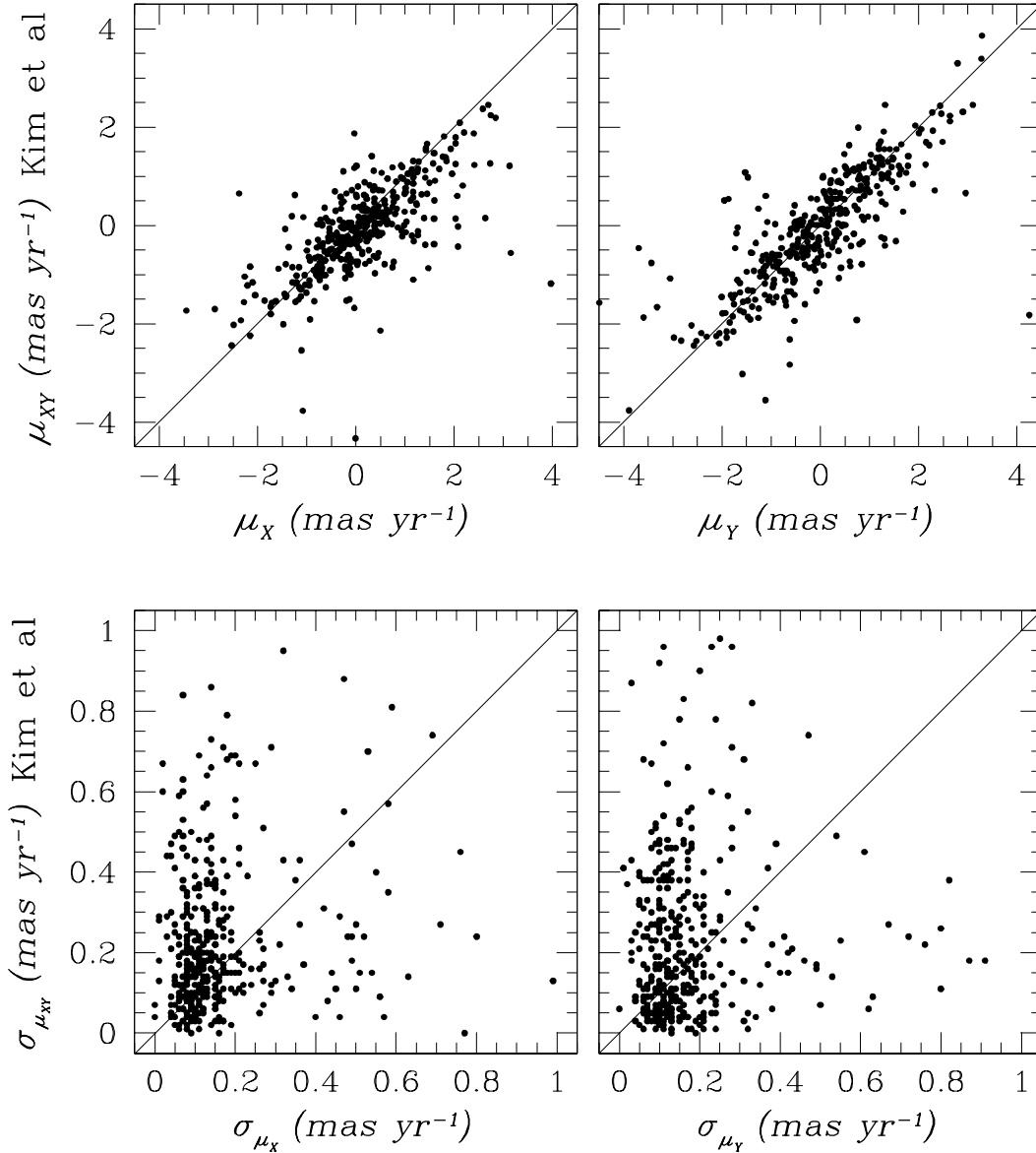
Figure 6. Comparison of proper motions and their errors between this study and that by Kim et al. (2019) . While the proper motions are distinctly commensurated, the corresponding distributions of proper-motion errors are lopsided.
