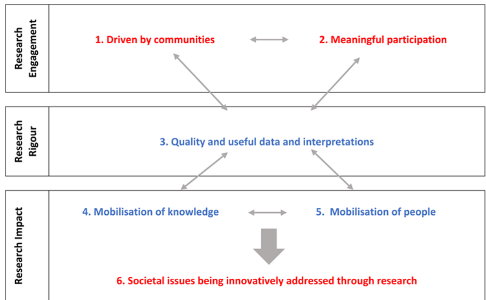
Figure 1 CBRET Theoretical Framework
